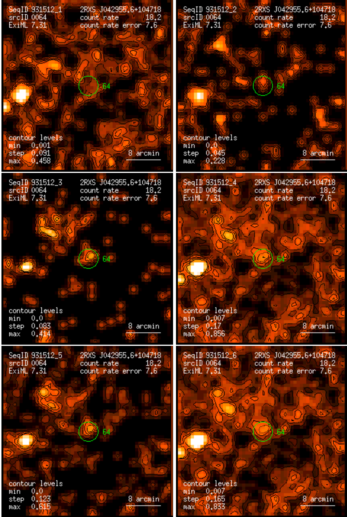
Figure 64: RASS 931512: detection 0064: band rate images, Gaussian filter: (1) PSPC channels 11 – 41, (2) 52 – 90, (3) 91 – 201, (4) 11 – 235, (5) 52 – 201, (6) 11 – 201. Broad band rates in counts/ks. Band rate contour levels in counts/ks/arcmin 2 .
