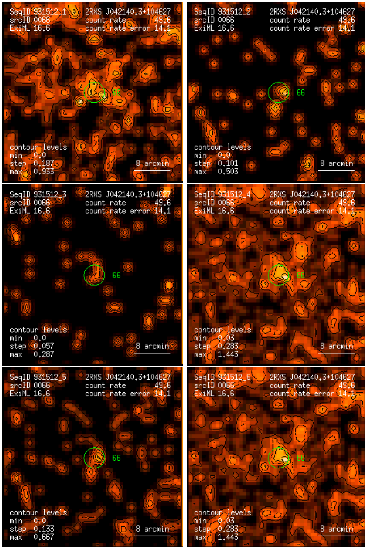
Figure 66: RASS 931512: detection 0066: band rate images, Gaussian filter: (1) PSPC channels 11 – 41, (2) 52 – 90, (3) 91 – 201, (4) 11 – 235, (5) 52 – 201, (6) 11 – 201. Broad band rates in counts/ks. Band rate contour levels in counts/ks/arcmin 2 .
