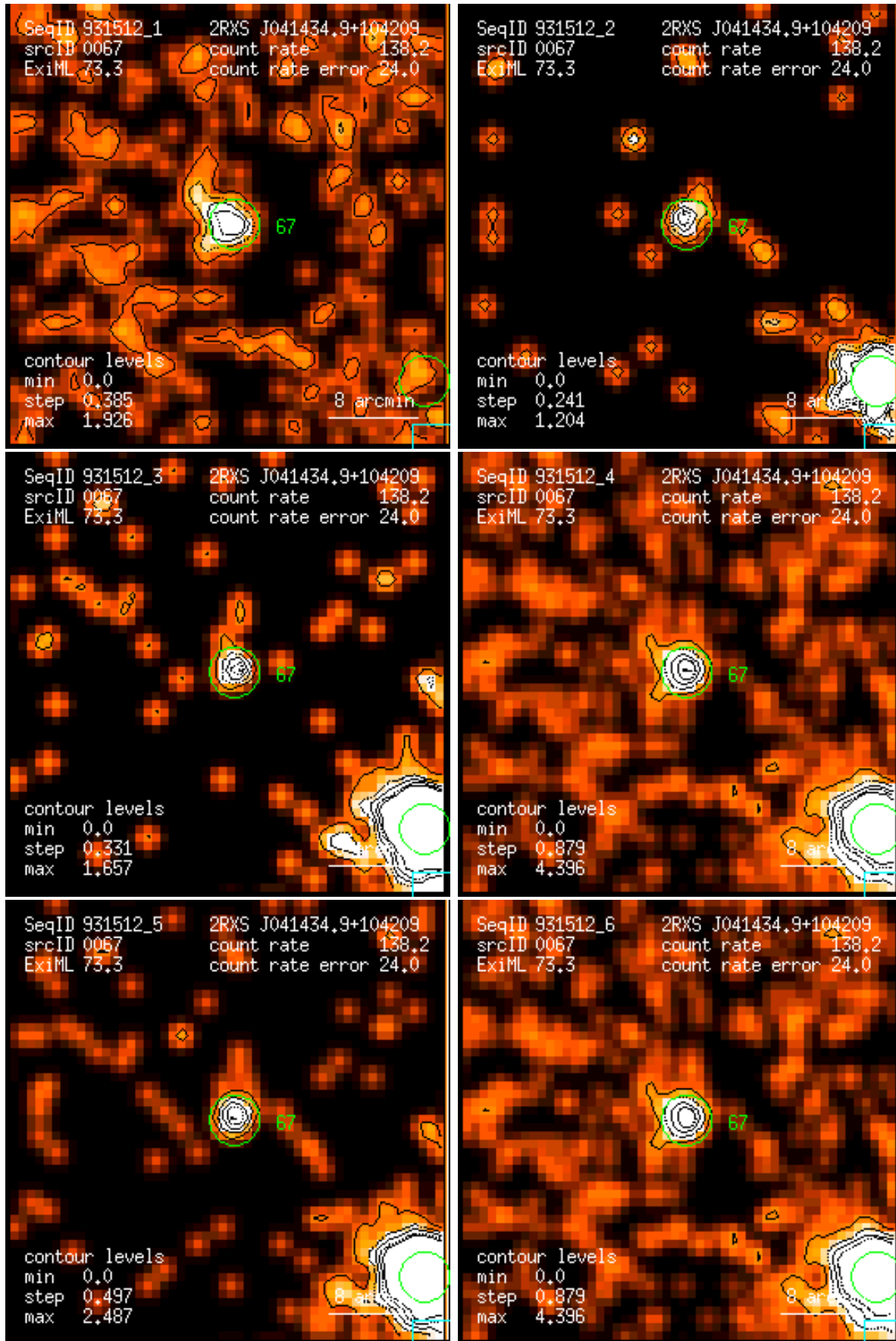
Figure 67: RASS 931512: detection 0067: band rate images, Gaussian filter: (1) PSPC channels 11 – 41, (2) 52 – 90, (3) 91 – 201, (4) 11 – 235, (5) 52 – 201, (6) 11 – 201. Broad band rates in counts/ks. Band rate contour levels in counts/ks/arcmin 2 .
