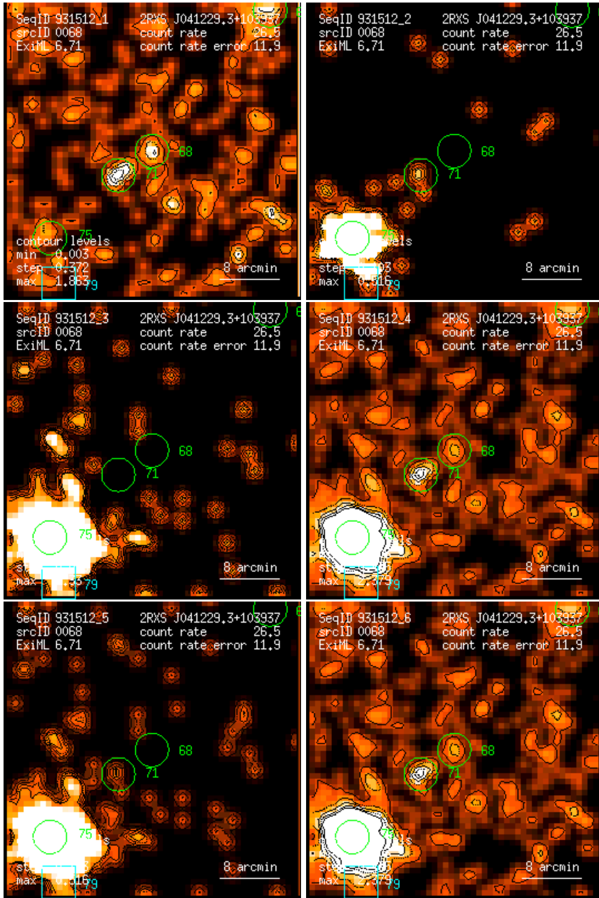
Figure 68: RASS 931512: detection 0068: band rate images, Gaussian filter: (1) PSPC channels 11 – 41, (2) 52 – 90, (3) 91 – 201, (4) 11 – 235, (5) 52 – 201, (6) 11 – 201. Broad band rates in counts/ks. Band rate contour levels in counts/ks/arcmin 2 .
