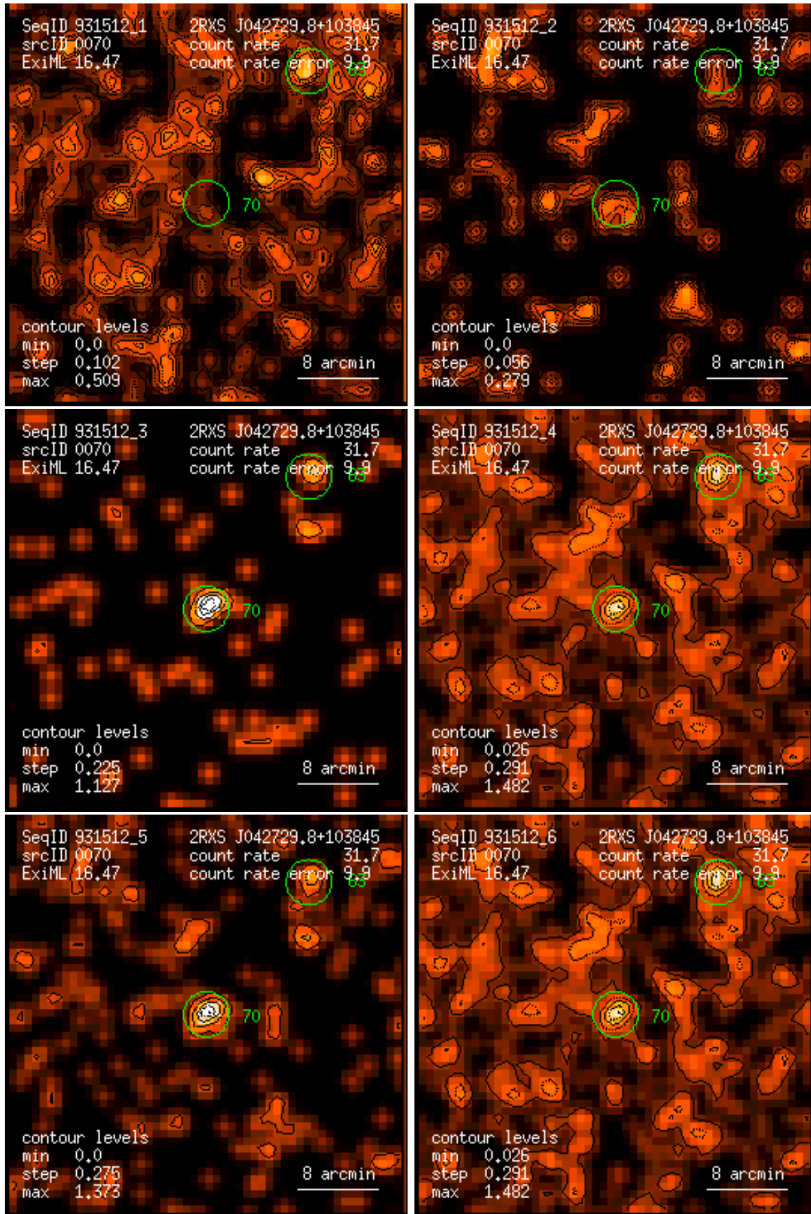
Figure 70: RASS 931512: detection 0070: band rate images, Gaussian filter: (1) PSPC channels 11 – 41, (2) 52 – 90, (3) 91 – 201, (4) 11 – 235, (5) 52 – 201, (6) 11 – 201. Broad band rates in counts/ks. Band rate contour levels in counts/ks/arcmin 2 .
