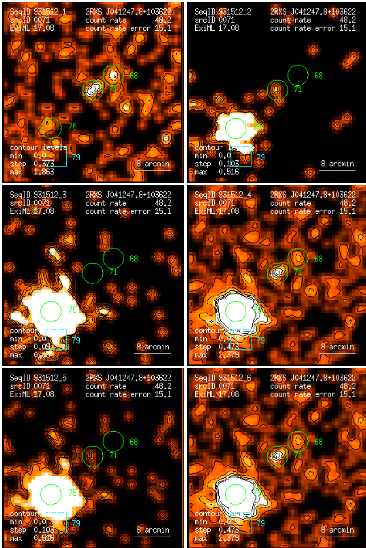
Figure 71: RASS 931512: detection 0071: band rate images, Gaussian filter: (1) PSPC channels 11 – 41, (2) 52 – 90, (3) 91 – 201, (4) 11 – 235, (5) 52 – 201, (6) 11 – 201. Broad band rates in counts/ks. Band rate contour levels in counts/ks/arcmin 2 .
