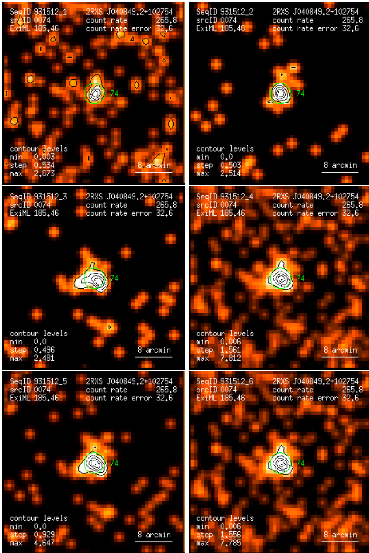
Figure 74: RASS 931512: detection 0074: band rate images, Gaussian filter: (1) PSPC channels 11 – 41, (2) 52 – 90, (3) 91 – 201, (4) 11 – 235, (5) 52 – 201, (6) 11 – 201. Broad band rates in counts/ks. Band rate contour levels in counts/ks/arcmin 2 .
