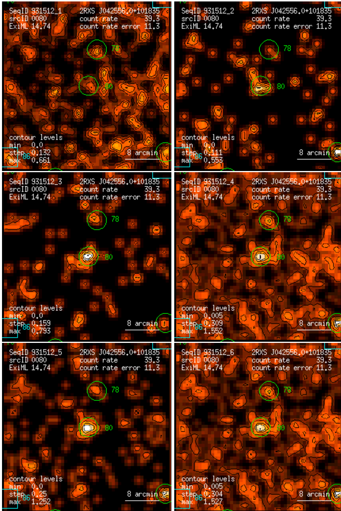
Figure 80: RASS 931512: detection 0080: band rate images, Gaussian filter: (1) PSPC channels 11 – 41, (2) 52 – 90, (3) 91 – 201, (4) 11 – 235, (5) 52 – 201, (6) 11 – 201. Broad band rates in counts/ks. Band rate contour levels in counts/ks/arcmin 2 .
