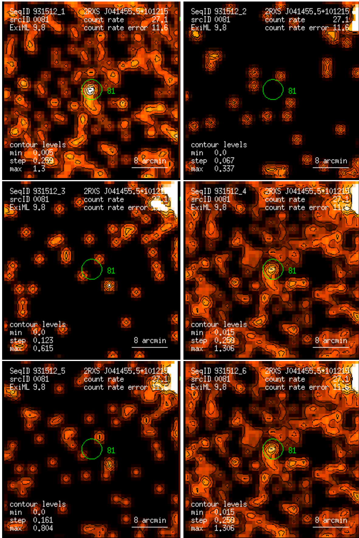
Figure 81: RASS 931512: detection 0081: band rate images, Gaussian filter: (1) PSPC channels 11 – 41, (2) 52 – 90, (3) 91 – 201, (4) 11 – 235, (5) 52 – 201, (6) 11 – 201. Broad band rates in counts/ks. Band rate contour levels in counts/ks/arcmin 2 .
