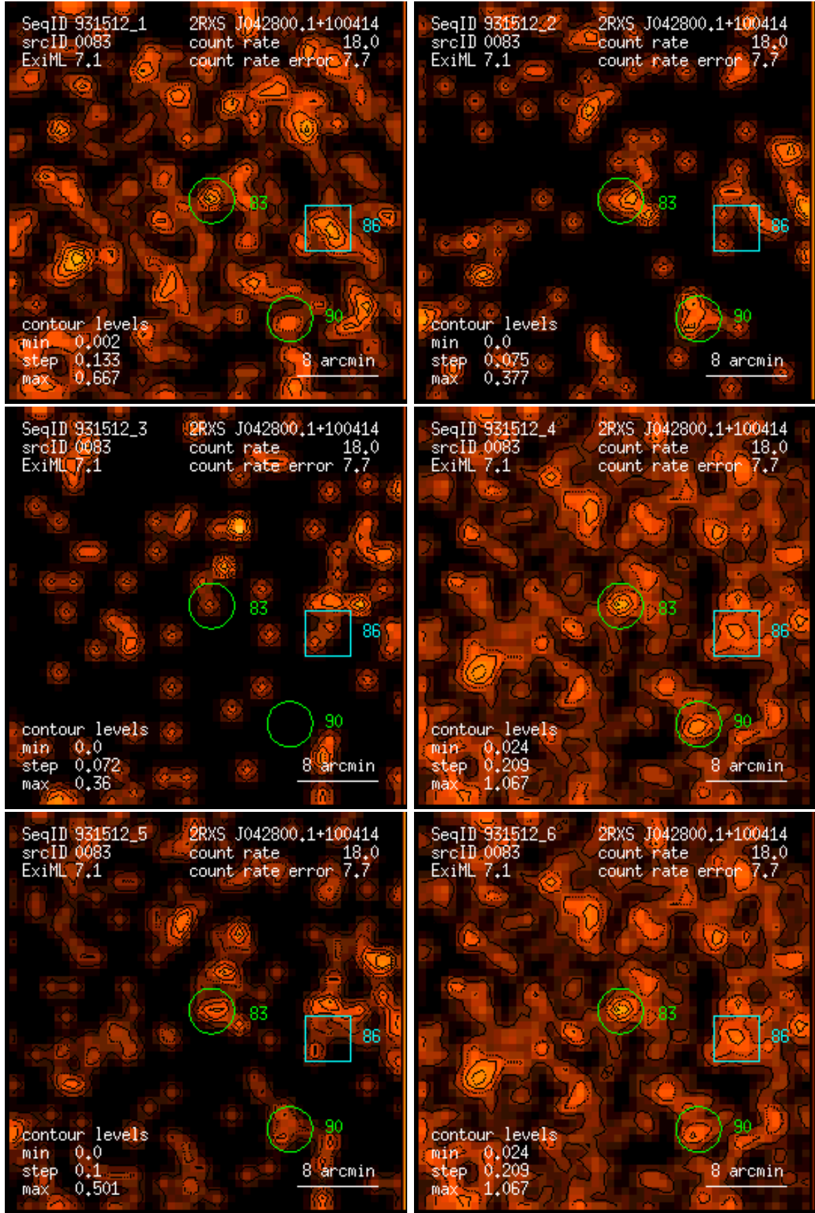
Figure 83: RASS 931512: detection 0083: band rate images, Gaussian filter: (1) PSPC channels 11 – 41, (2) 52 – 90, (3) 91 – 201, (4) 11 – 235, (5) 52 – 201, (6) 11 – 201. Broad band rates in counts/ks. Band rate contour levels in counts/ks/arcmin 2 .
