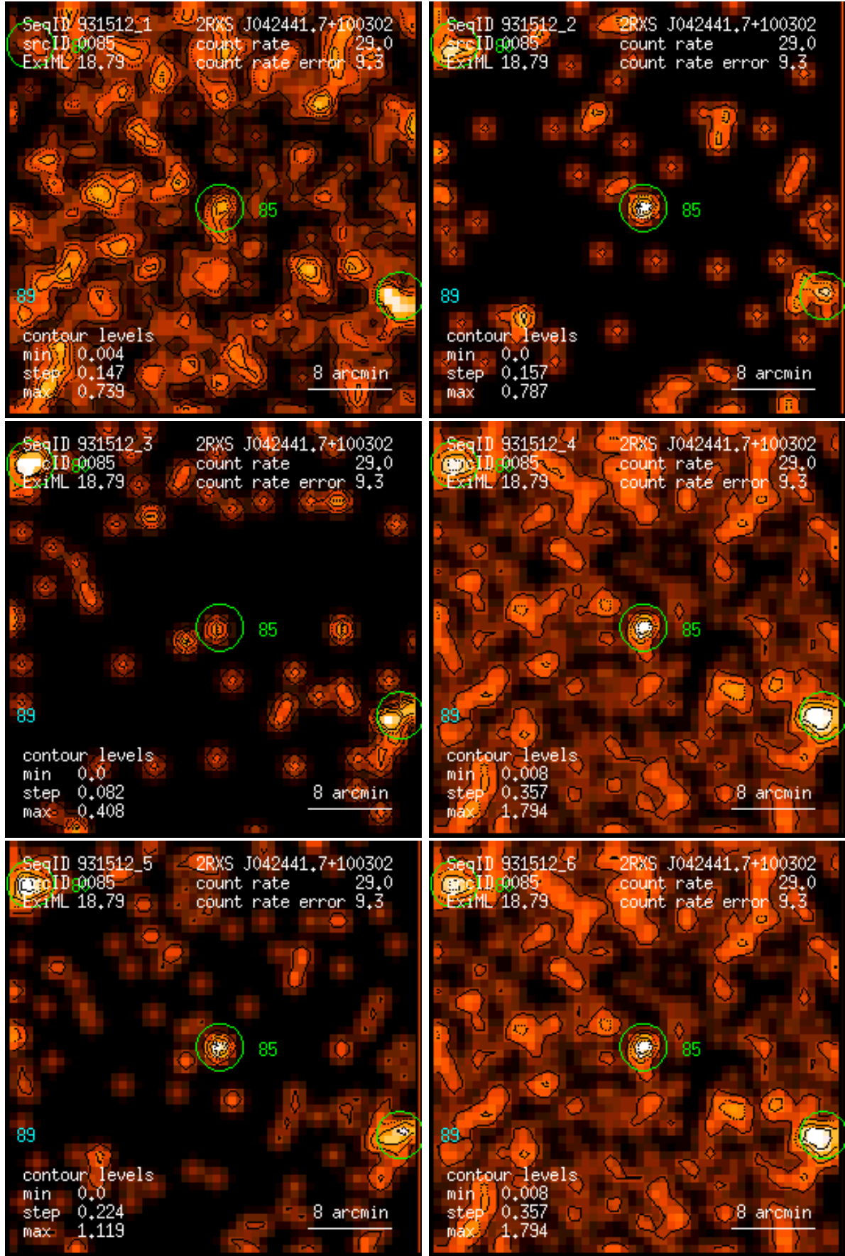
Figure 85: RASS 931512: detection 0085: band rate images, Gaussian filter: (1) PSPC channels 11 – 41, (2) 52 – 90, (3) 91 – 201, (4) 11 – 235, (5) 52 – 201, (6) 11 – 201. Broad band rates in counts/ks. Band rate contour levels in counts/ks/arcmin 2 .
