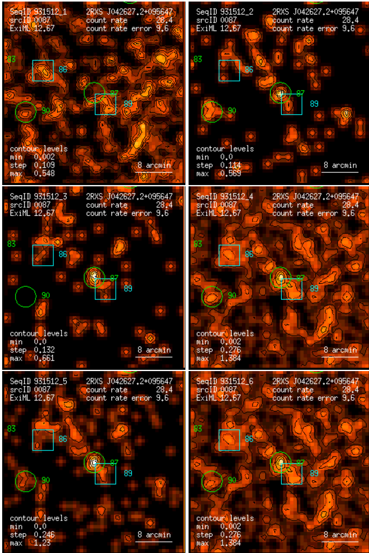
Figure 87: RASS 931512: detection 0087: band rate images, Gaussian filter: (1) PSPC channels 11 – 41, (2) 52 – 90, (3) 91 – 201, (4) 11 – 235, (5) 52 – 201, (6) 11 – 201. Broad band rates in counts/ks. Band rate contour levels in counts/ks/arcmin 2 .
