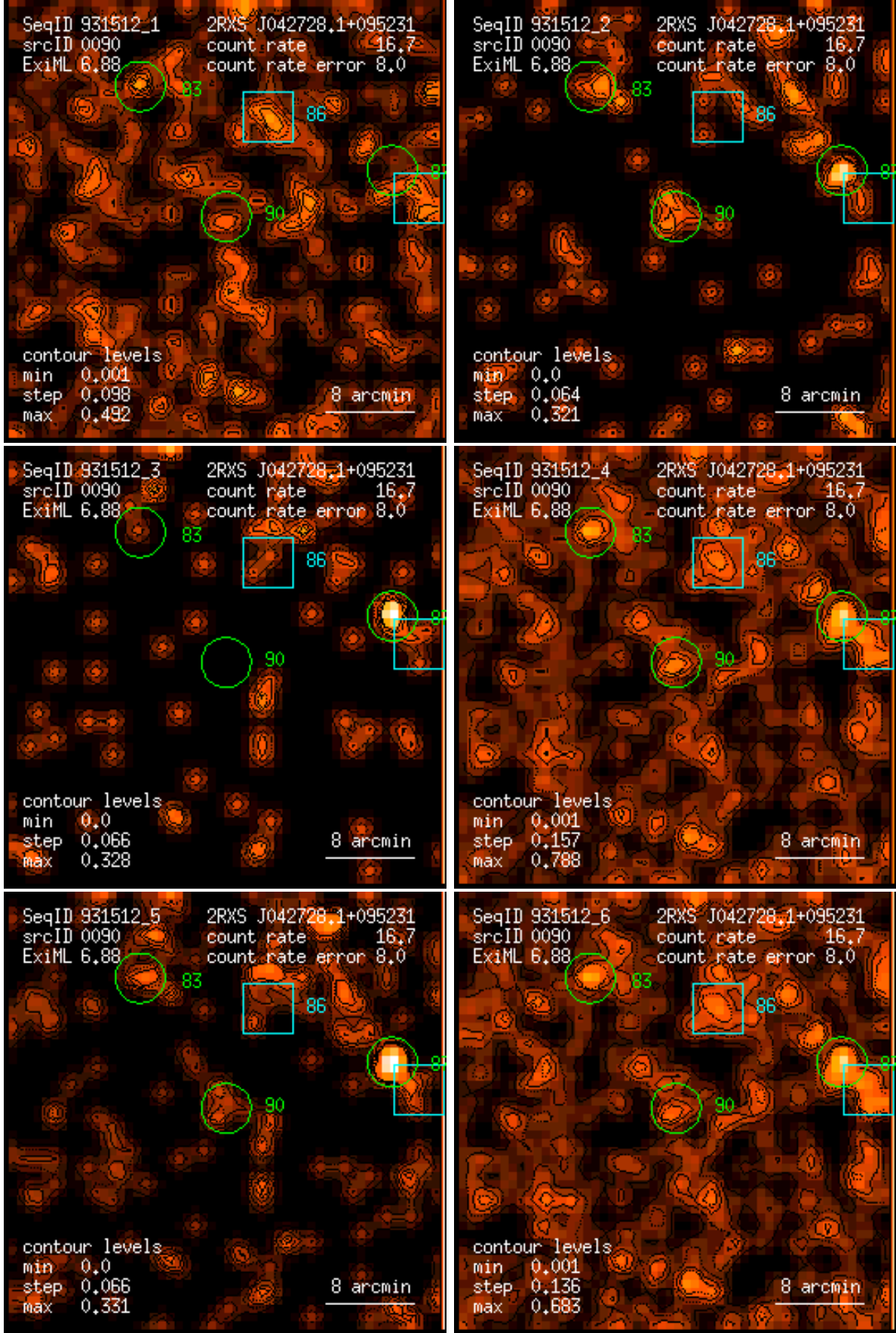
Figure 90: RASS 931512: detection 0090: band rate images, Gaussian filter: (1) PSPC channels 11 – 41, (2) 52 – 90, (3) 91 – 201, (4) 11 – 235, (5) 52 – 201, (6) 11 – 201. Broad band rates in counts/ks. Band rate contour levels in counts/ks/arcmin 2 .
