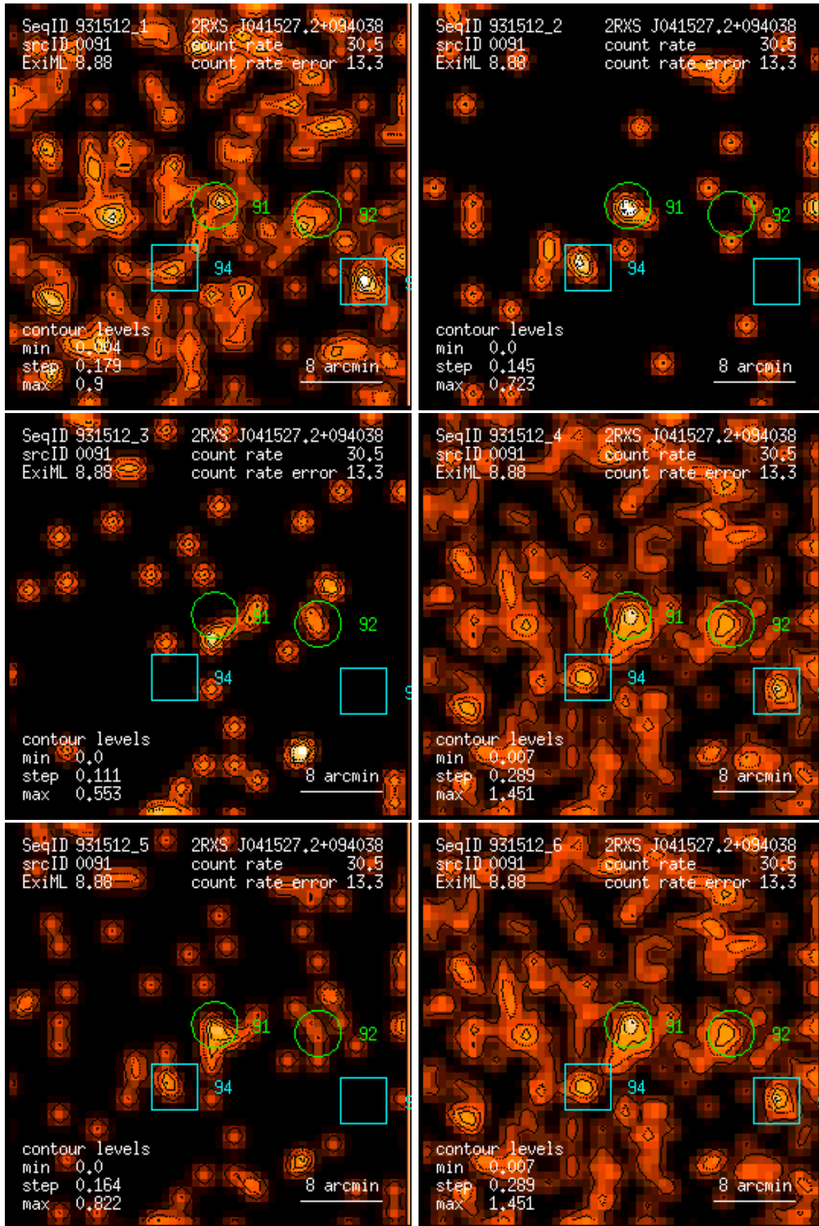
Figure 91: RASS 931512: detection 0091: band rate images, Gaussian filter: (1) PSPC channels 11 – 41, (2) 52 – 90, (3) 91 – 201, (4) 11 – 235, (5) 52 – 201, (6) 11 – 201. Broad band rates in counts/ks. Band rate contour levels in counts/ks/arcmin 2 .
