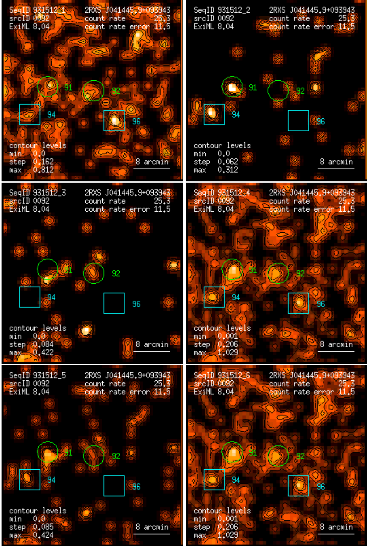
Figure 92: RASS 931512: detection 0092: band rate images, Gaussian filter: (1) PSPC channels 11 – 41, (2) 52 – 90, (3) 91 – 201, (4) 11 – 235, (5) 52 – 201, (6) 11 – 201. Broad band rates in counts/ks. Band rate contour levels in counts/ks/arcmin 2 .
