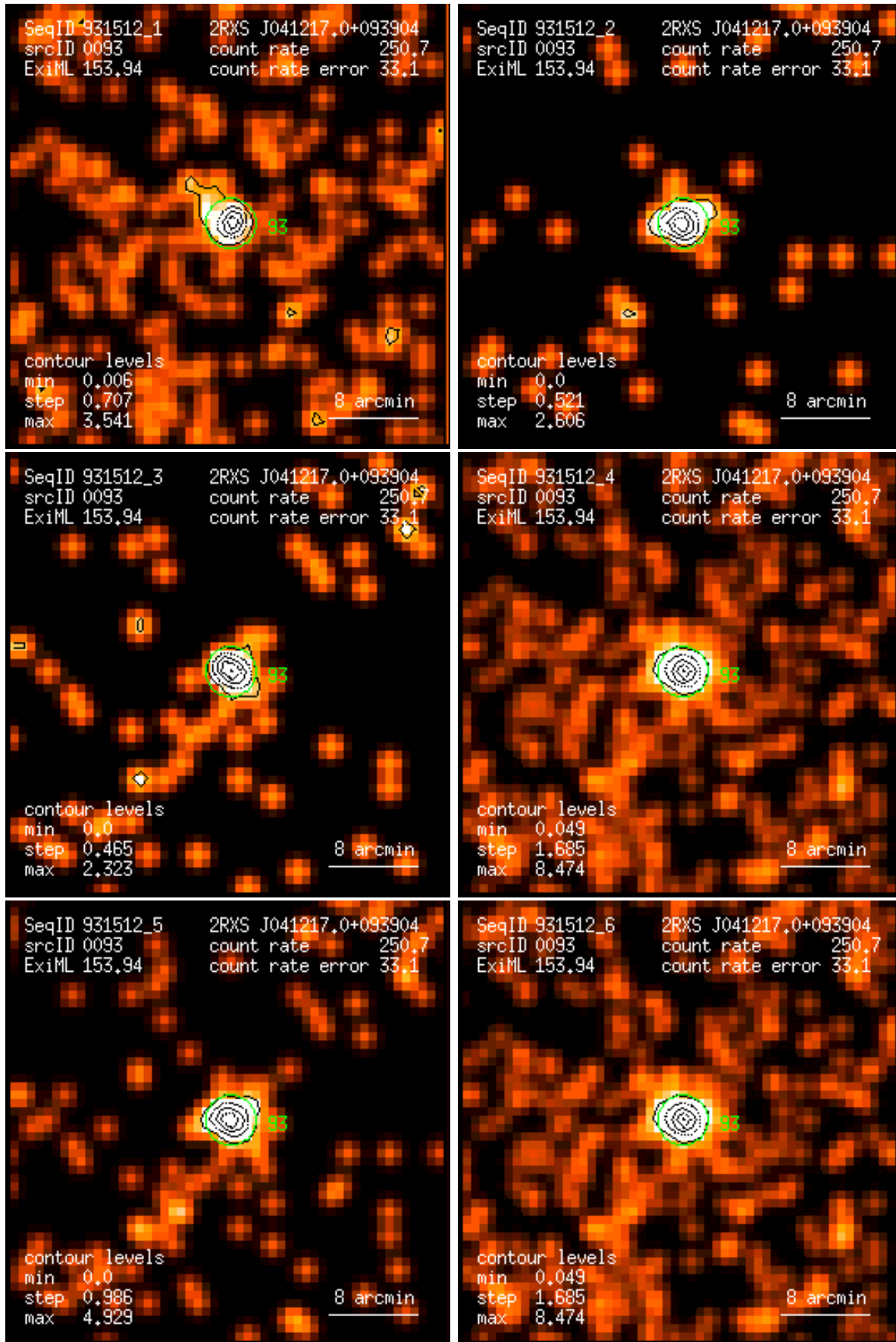
Figure 93: RASS 931512: detection 0093: band rate images, Gaussian filter: (1) PSPC channels 11 – 41, (2) 52 – 90, (3) 91 – 201, (4) 11 – 235, (5) 52 – 201, (6) 11 – 201. Broad band rates in counts/ks. Band rate contour levels in counts/ks/arcmin 2 .
