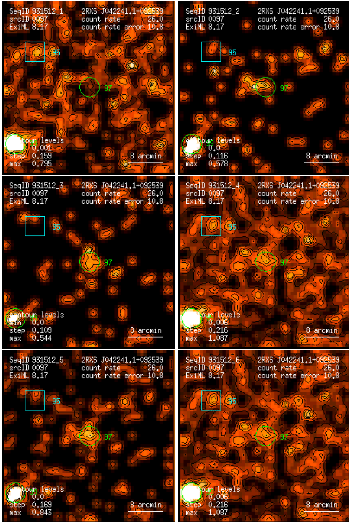
Figure 97: RASS 931512: detection 0097: band rate images, Gaussian filter: (1) PSPC channels 11 – 41, (2) 52 – 90, (3) 91 – 201, (4) 11 – 235, (5) 52 – 201, (6) 11 – 201. Broad band rates in counts/ks. Band rate contour levels in counts/ks/arcmin 2 .
