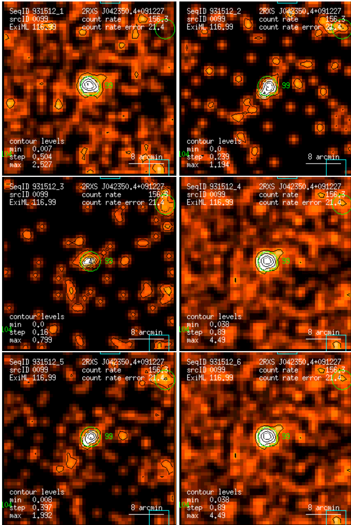
Figure 99: RASS 931512: detection 0099: band rate images, Gaussian filter: (1) PSPC channels 11 – 41, (2) 52 – 90, (3) 91 – 201, (4) 11 – 235, (5) 52 – 201, (6) 11 – 201. Broad band rates in counts/ks. Band rate contour levels in counts/ks/arcmin 2 .
