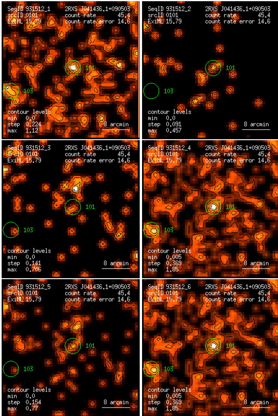
Figure 101: RASS 931512: detection 0101: band rate images, Gaussian filter: (1) PSPC channels 11 – 41, (2) 52 – 90, (3) 91 – 201, (4) 11 – 235, (5) 52 – 201, (6) 11 – 201. Broad band rates in counts/ks. Band rate contour levels in counts/ks/arcmin 2 .
