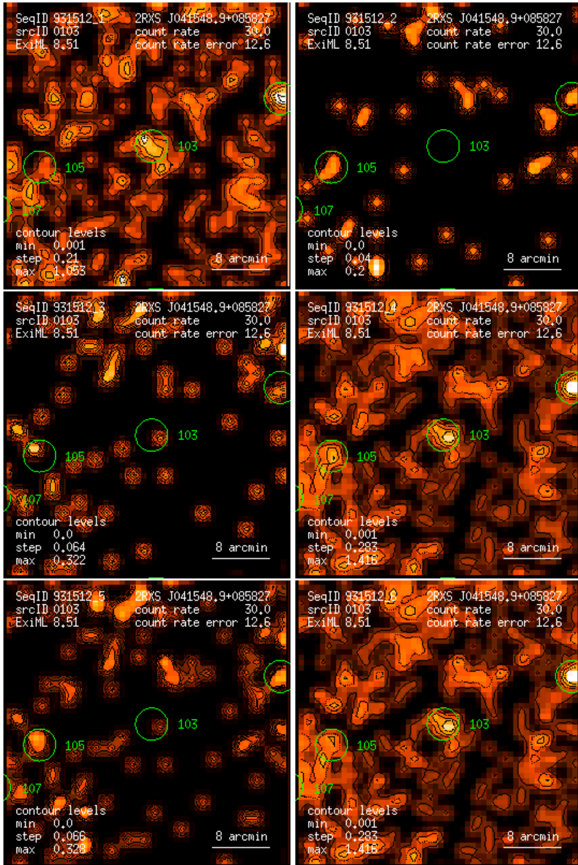
Figure 103: RASS 931512: detection 0103: band rate images, Gaussian filter: (1) PSPC channels 11 – 41, (2) 52 – 90, (3) 91 – 201, (4) 11 – 235, (5) 52 – 201, (6) 11 – 201. Broad band rates in counts/ks. Band rate contour levels in counts/ks/arcmin 2 .
