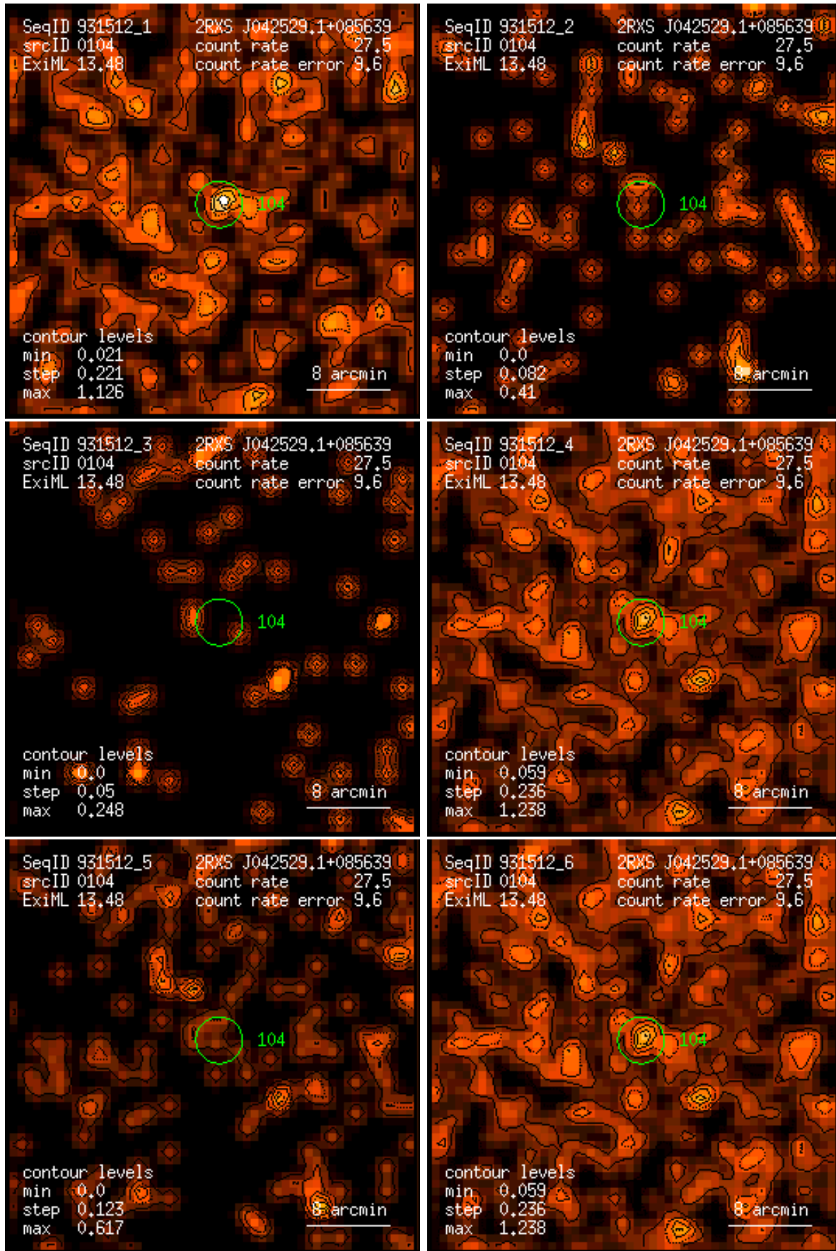
Figure 104: RASS 931512: detection 0104: band rate images, Gaussian filter: (1) PSPC channels 11 – 41, (2) 52 – 90, (3) 91 – 201, (4) 11 – 235, (5) 52 – 201, (6) 11 – 201. Broad band rates in counts/ks. Band rate contour levels in counts/ks/arcmin 2 .
