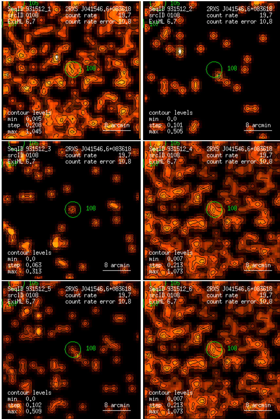
Figure 108: RASS 931512: detection 0108: band rate images, Gaussian filter: (1) PSPC channels 11 – 41, (2) 52 – 90, (3) 91 – 201, (4) 11 – 235, (5) 52 – 201, (6) 11 – 201. Broad band rates in counts/ks. Band rate contour levels in counts/ks/arcmin 2 .
