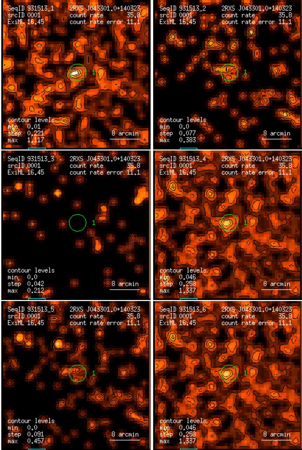
Figure 1: RASS 931513: detection 0001: band rate images, Gaussian filter: (1) PSPC channels 11 – 41, (2) 52 – 90, (3) 91 – 201, (4) 11 – 235, (5) 52 – 201, (6) 11 – 201. Broad band rates in counts/ks. Band rate contour levels in counts/ks/arcmin 2 .
