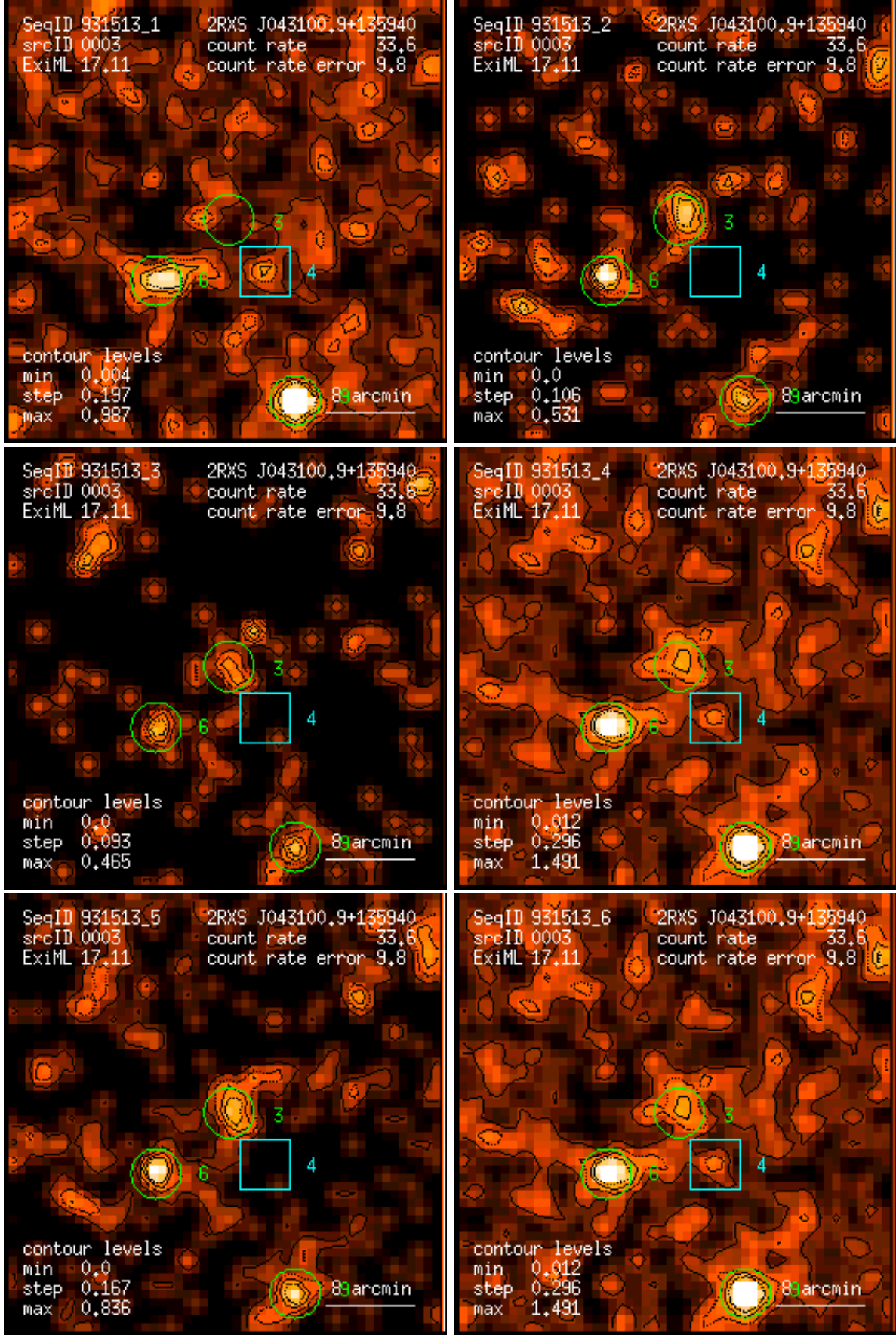
Figure 3: RASS 931513: detection 0003: band rate images, Gaussian filter: (1) PSPC channels 11 – 41, (2) 52 – 90, (3) 91 – 201, (4) 11 – 235, (5) 52 – 201, (6) 11 – 201. Broad band rates in counts/ks. Band rate contour levels in counts/ks/arcmin 2 .
