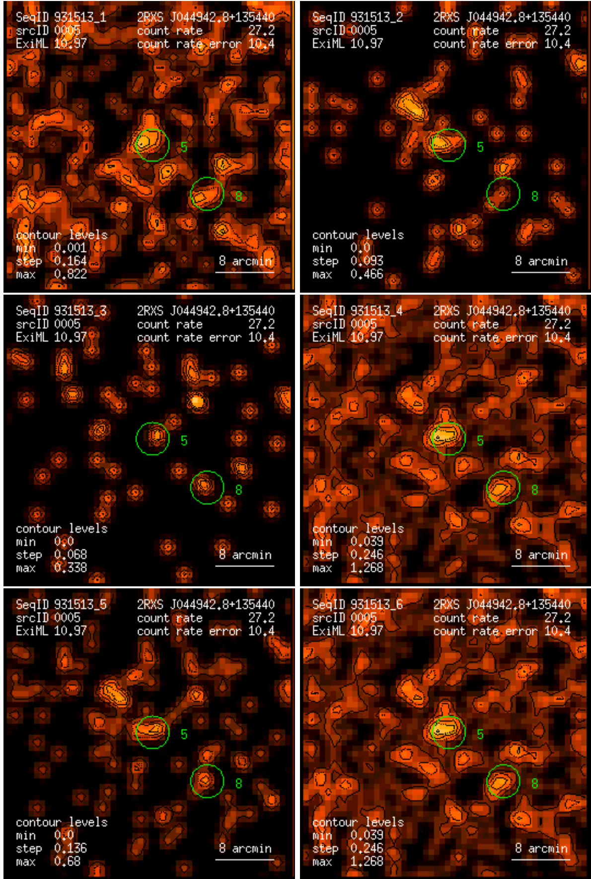
Figure 5: RASS 931513: detection 0005: band rate images, Gaussian filter: (1) PSPC channels 11 – 41, (2) 52 – 90, (3) 91 – 201, (4) 11 – 235, (5) 52 – 201, (6) 11 – 201. Broad band rates in counts/ks. Band rate contour levels in counts/ks/arcmin 2 .
