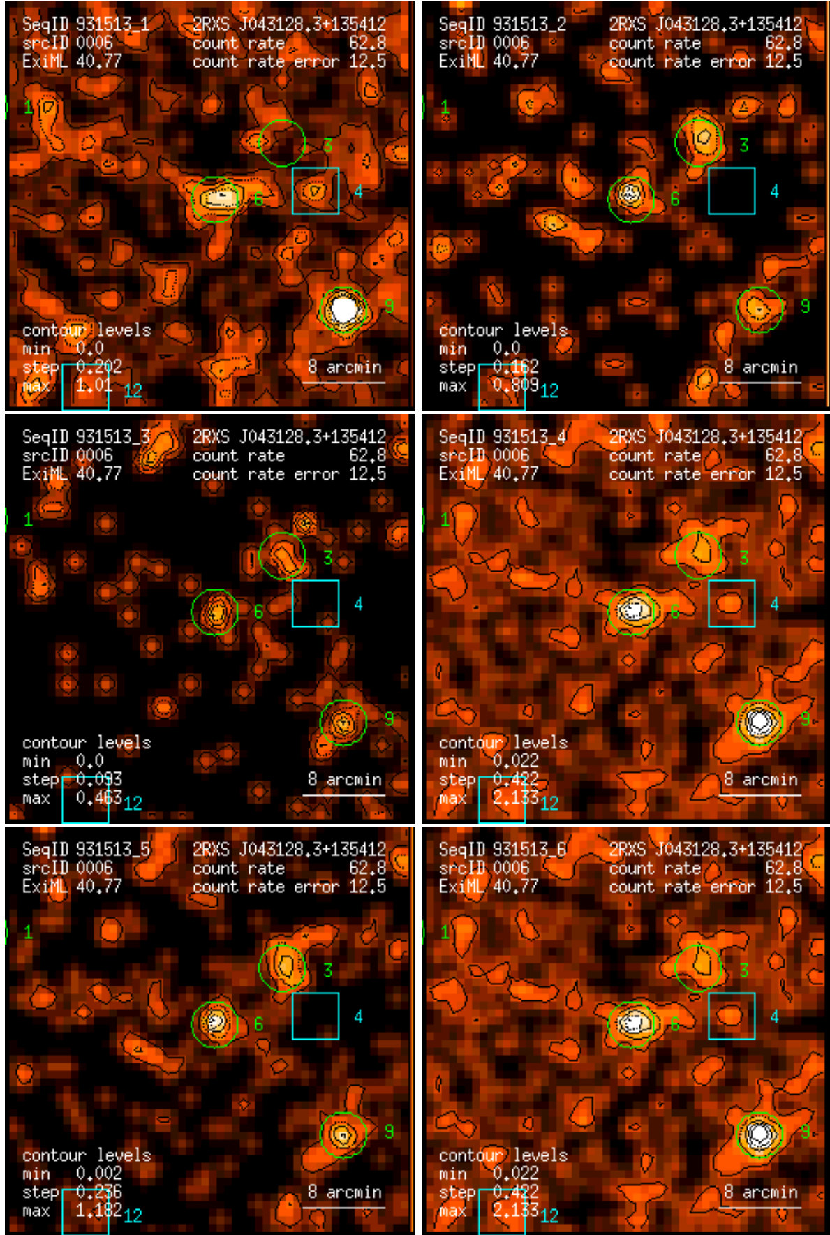
Figure 6: RASS 931513: detection 0006: band rate images, Gaussian filter: (1) PSPC channels 11 – 41, (2) 52 – 90, (3) 91 – 201, (4) 11 – 235, (5) 52 – 201, (6) 11 – 201. Broad band rates in counts/ks. Band rate contour levels in counts/ks/arcmin 2 .
