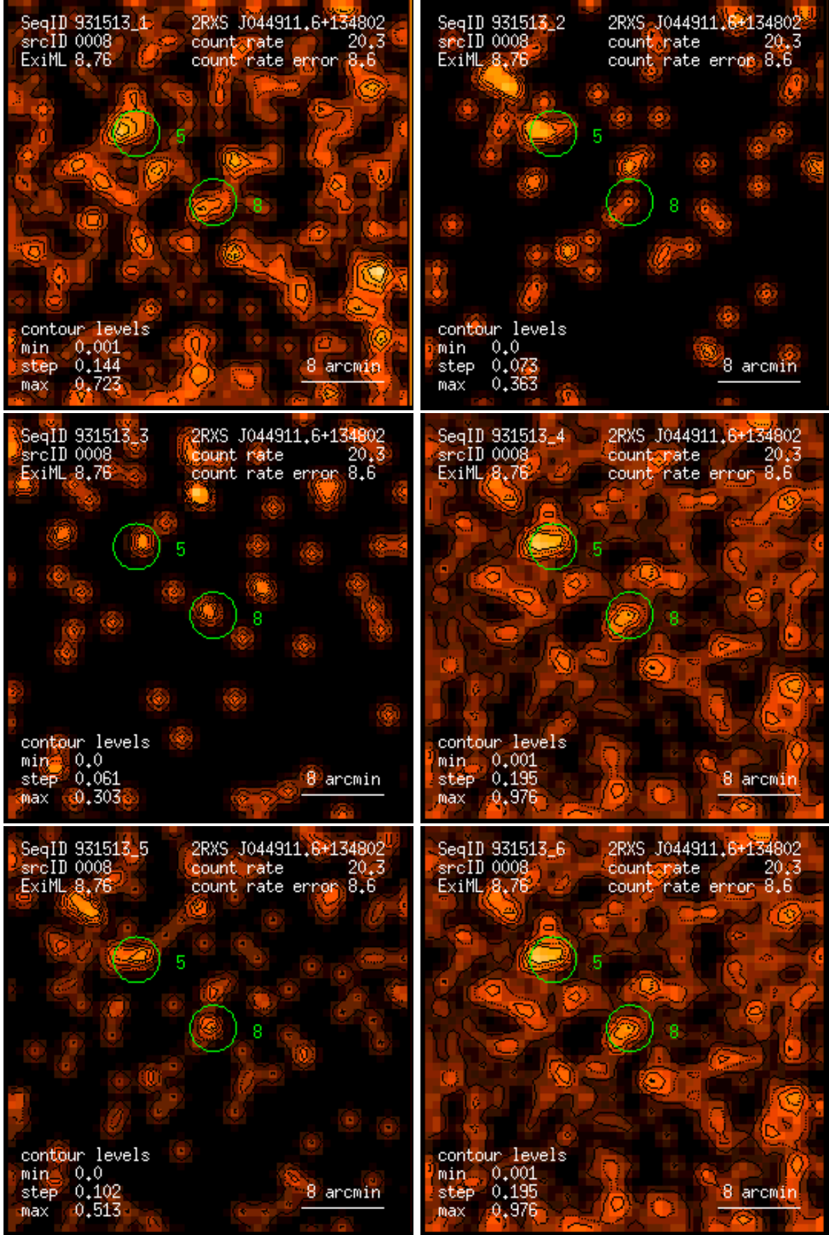
Figure 8: RASS 931513: detection 0008: band rate images, Gaussian filter: (1) PSPC channels 11 – 41, (2) 52 – 90, (3) 91 – 201, (4) 11 – 235, (5) 52 – 201, (6) 11 – 201. Broad band rates in counts/ks. Band rate contour levels in counts/ks/arcmin 2 .
