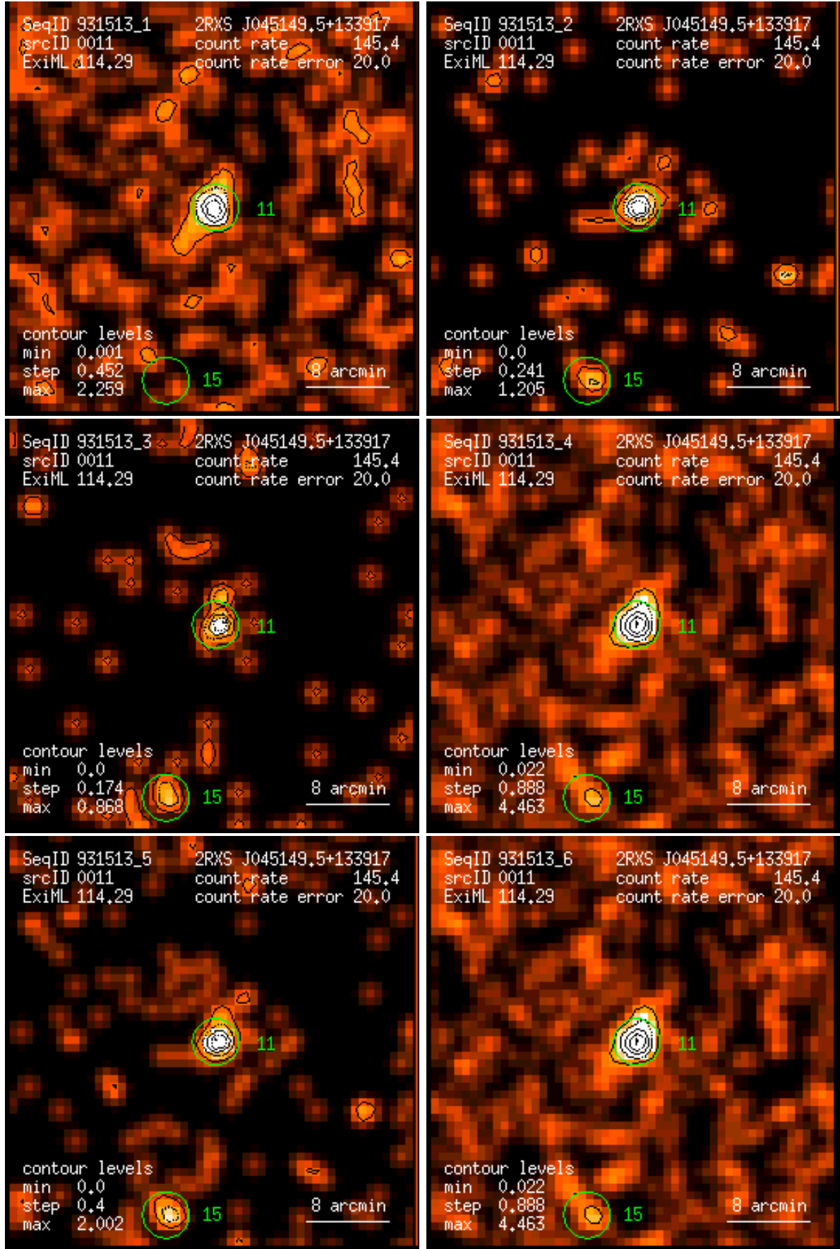
Figure 11: RASS 931513: detection 0011: band rate images, Gaussian filter: (1) PSPP channels 11 – 41, (2) 52 – 90, (3) 91 – 201, (4) 11 – 235, (5) 52 – 201, (6) 11 – 201. Broad band rates in counts/ks. Band rate contour levels in counts/ks/arcmin 2 .
