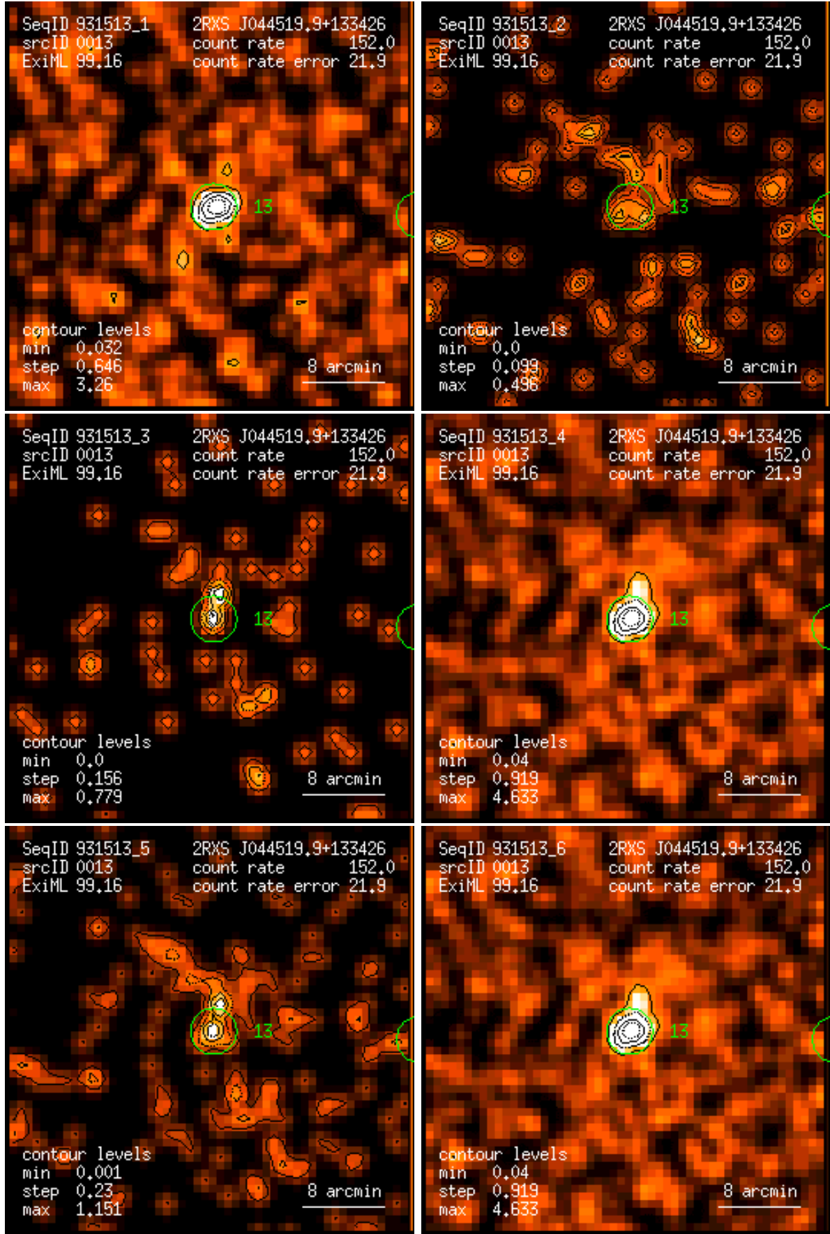
Figure 13: RASS 931513: detection 0013: band rate images, Gaussian filter: (1) PSPC channels 11 – 41, (2) 52 – 90, (3) 91 – 201, (4) 11 – 235, (5) 52 – 201, (6) 11 – 201. Broad band rates in counts/ks. Band rate contour levels in counts/ks/arcmin 2 .
