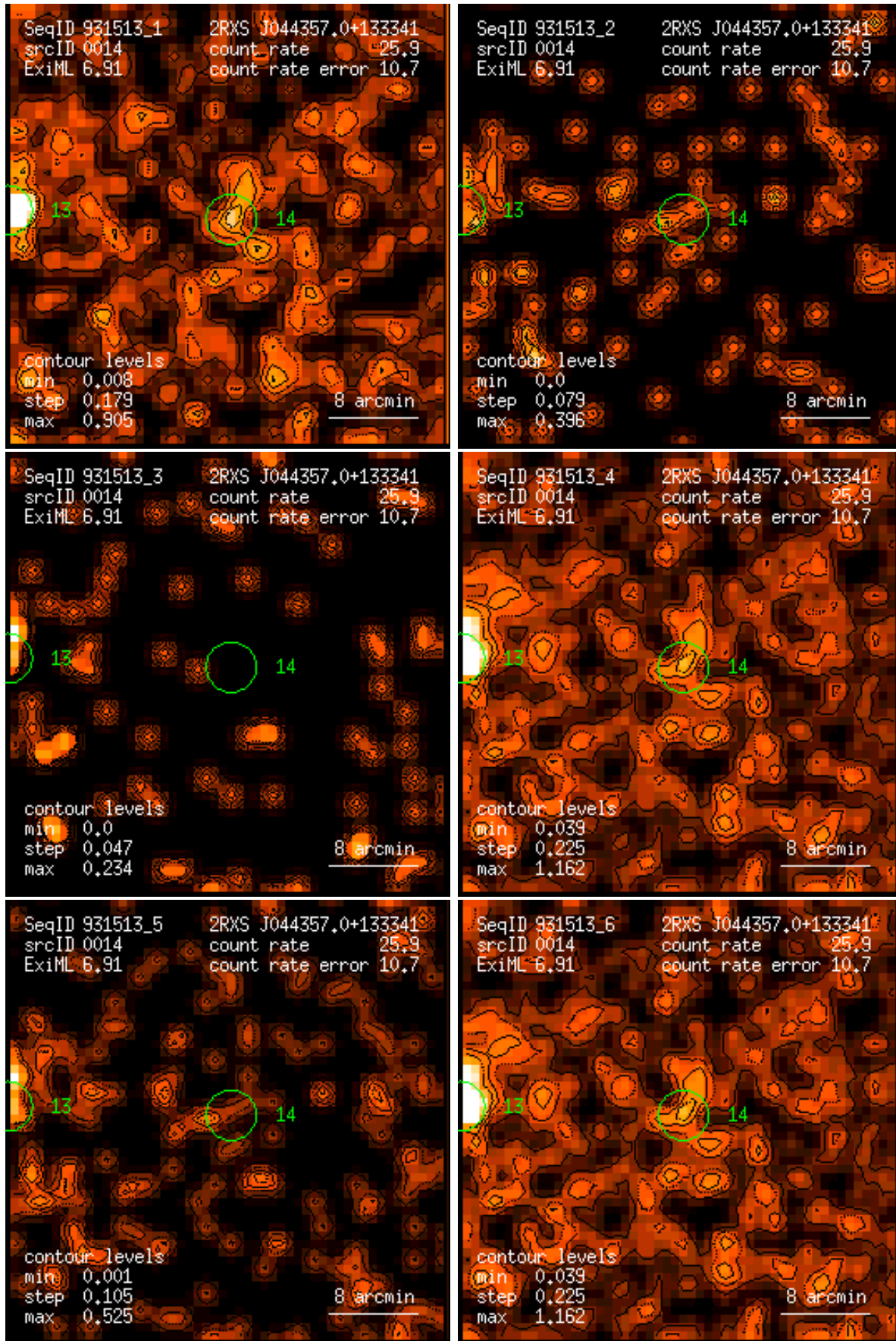
Figure 14: RASS 931513: detection 0014: band rate images, Gaussian filter: (1) PSPC channels 11 – 41, (2) 52 – 90, (3) 91 – 201, (4) 11 – 235, (5) 52 – 201, (6) 11 – 201. Broad band rates in counts/ks. Band rate contour levels in counts/ks/arcmin 2 .
