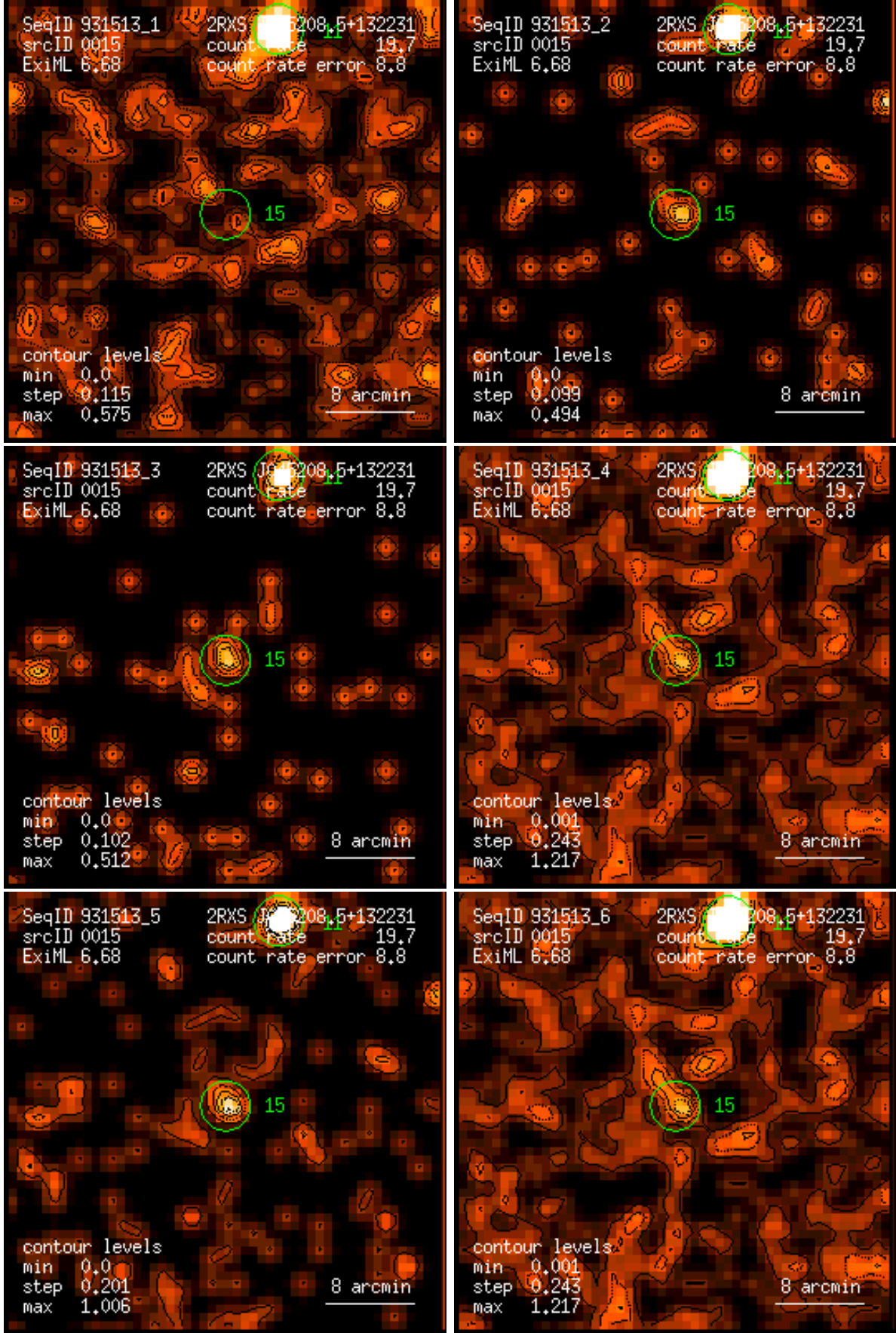
Figure 15: RASS 931513: detection 0015: band rate images, Gaussian filter: (1) PSPC channels 11 – 41, (2) 52 – 90, (3) 91 – 201, (4) 11 – 235, (5) 52 – 201, (6) 11 – 201. Broad band rates in counts/ks. Band rate contour levels in counts/ks/arcmin 2 .
