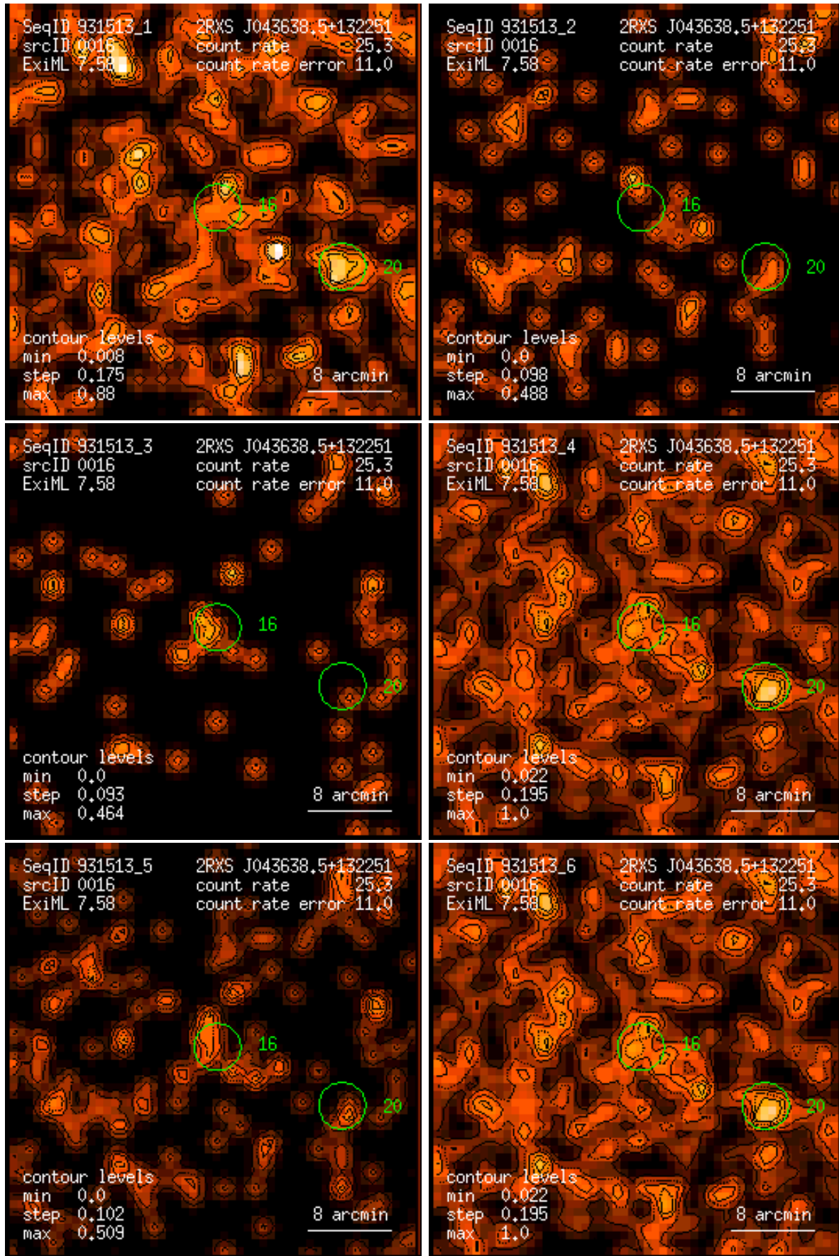
Figure 16: RASS 931513: detection 0016: band rate images, Gaussian filter: (1) PSPC channels 11 – 41, (2) 52 – 90, (3) 91 – 201, (4) 11 – 235, (5) 52 – 201, (6) 11 – 201. Broad band rates in counts/ks. Band rate contour levels in counts/ks/arcmin 2 .
