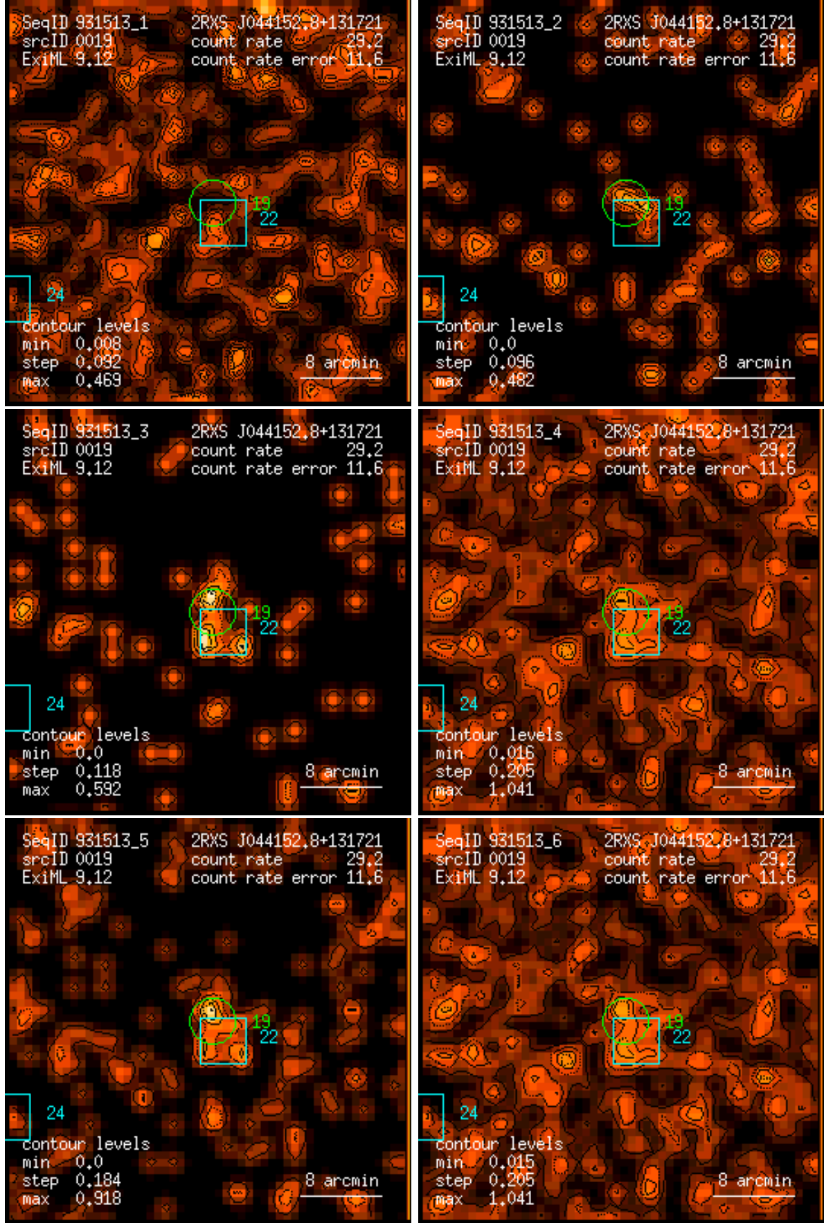
Figure 19: RASS 931513: detection 0019: band rate images, Gaussian filter: (1) PSPC channels 11 – 41, (2) 52 – 90, (3) 91 – 201, (4) 11 – 235, (5) 52 – 201, (6) 11 – 201. Broad band rates in counts/ks. Band rate contour levels in counts/ks/arcmin 2 .
