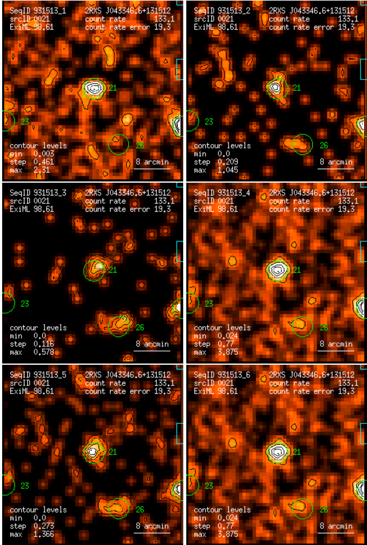
Figure 21: RASS 931513: detection 0021: band rate images, Gaussian filter: (1) PSPC channels 11 – 41, (2) 52 – 90, (3) 91 – 201, (4) 11 – 235, (5) 52 – 201, (6) 11 – 201. Broad band rates in counts/ks. Band rate contour levels in counts/ks/arcmin 2 .
