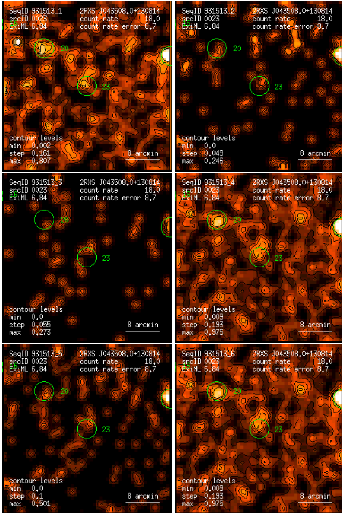
Figure 23: RASS 931513: detection 0023: band rate images, Gaussian filter: (1) PSPC channels 11 – 41, (2) 52 – 90, (3) 91 – 201, (4) 11 – 235, (5) 52 – 201, (6) 11 – 201. Broad band rates in counts/ks. Band rate contour levels in counts/ks/arcmin 2 .
