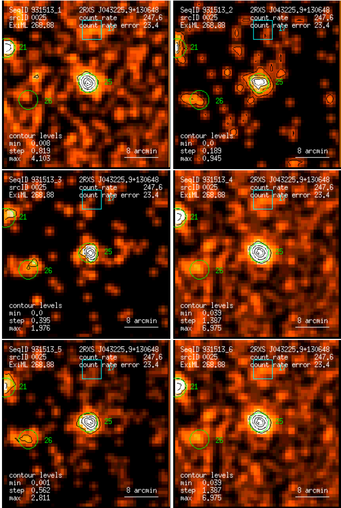
Figure 25: RASS 931513: detection 0025: band rate images, Gaussian filter: (1) PSPC channels 11 – 41, (2) 52 – 90, (3) 91 – 201, (4) 11 – 235, (5) 52 – 201, (6) 11 – 201. Broad band rates in counts/ks. Band rate contour levels in counts/ks/arcmin 2 .
