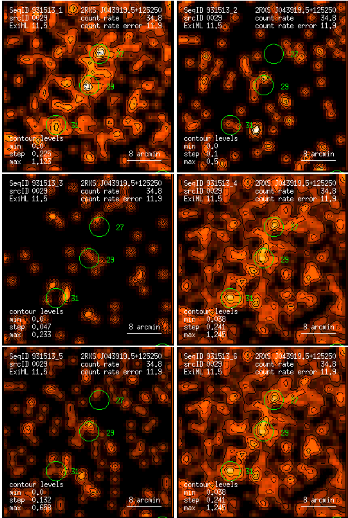
Figure 29: RASS 931513: detection 0029: band rate images, Gaussian filter: (1) PSPC channels 11 – 41, (2) 52 – 90, (3) 91 – 201, (4) 11 – 235, (5) 52 – 201, (6) 11 – 201. Broad band rates in counts/ks. Band rate contour levels in counts/ks/arcmin 2 .
