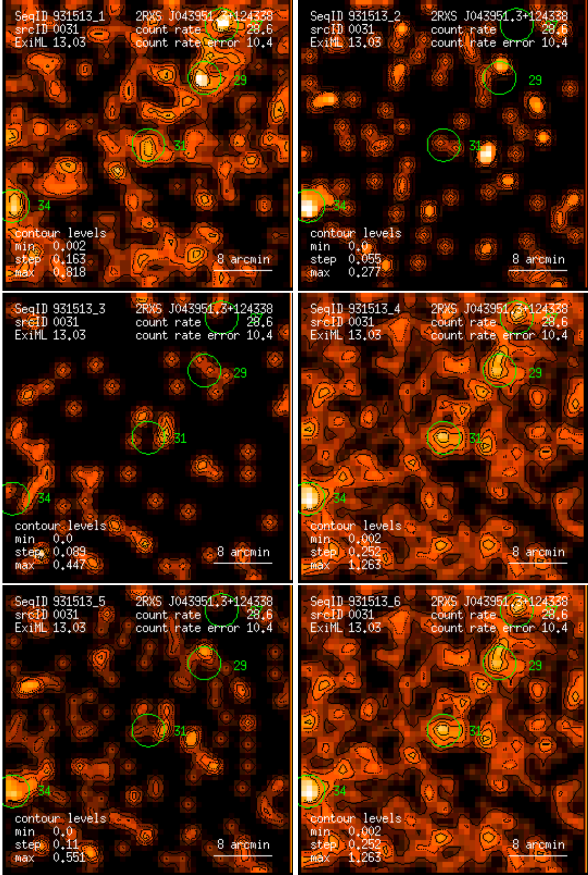
Figure 31: RASS 931513: detection 0031: band rate images, Gaussian filter: (1) PSPC channels 11 – 41, (2) 52 – 90, (3) 91 – 201, (4) 11 – 235, (5) 52 – 201, (6) 11 – 201. Broad band rates in counts/ks. Band rate contour levels in counts/ks/arcmin 2 .
