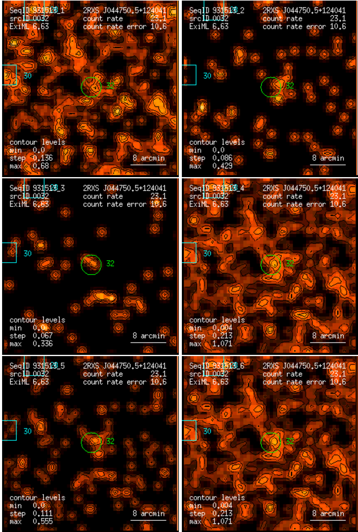
Figure 32: RASS 931513: detection 0032: band rate images, Gaussian filter: (1) PSPC channels 11 – 41, (2) 52 – 90, (3) 91 – 201, (4) 11 – 235, (5) 52 – 201, (6) 11 – 201. Broad band rates in counts/ks. Band rate contour levels in counts/ks/arcmin 2 .
