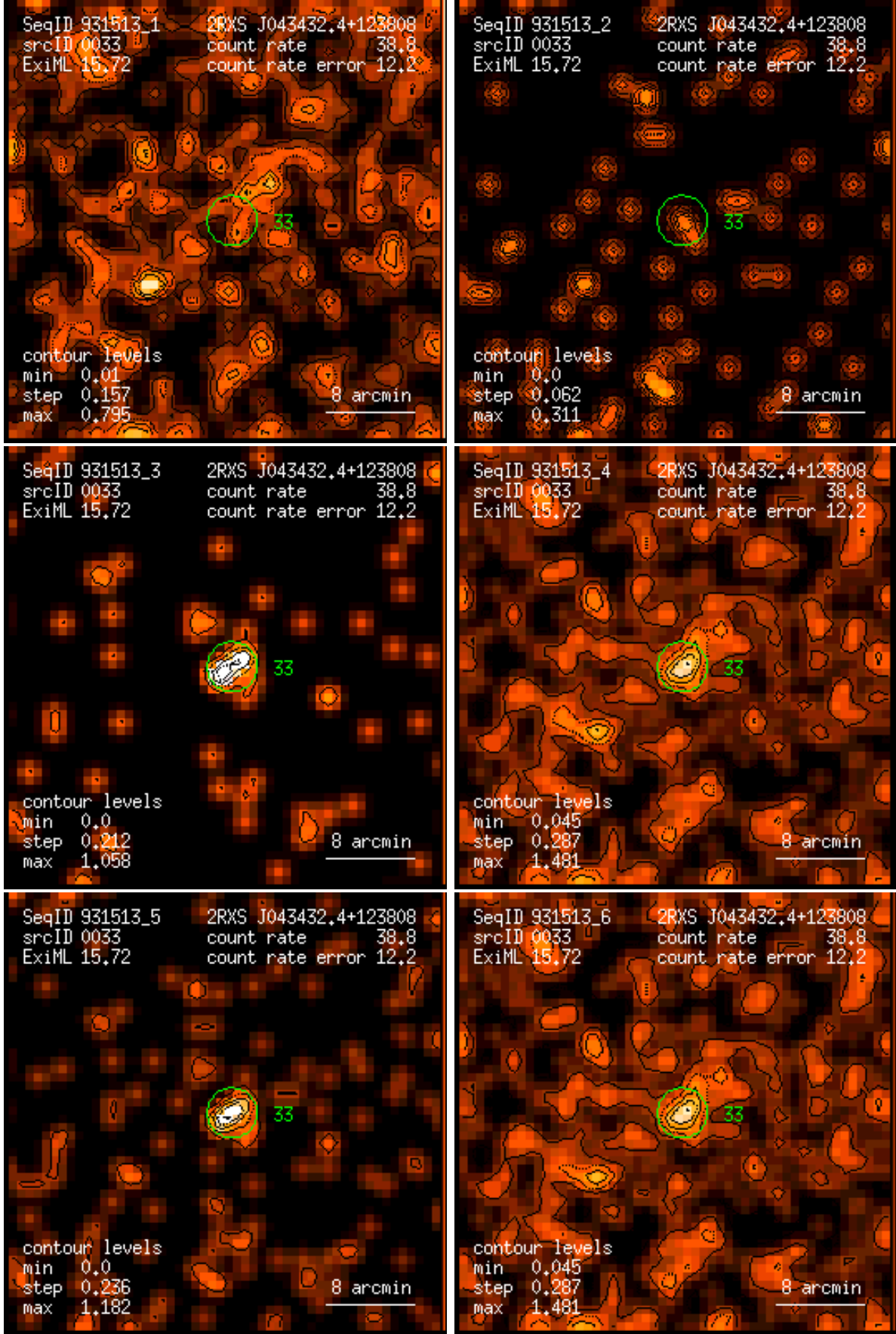
Figure 33: RASS 931513: detection 0033: band rate images, Gaussian filter: (1) PSPC channels 11 – 41, (2) 52 – 90, (3) 91 – 201, (4) 11 – 235, (5) 52 – 201, (6) 11 – 201. Broad band rates in counts/ks. Band rate contour levels in counts/ks/arcmin 2 .
