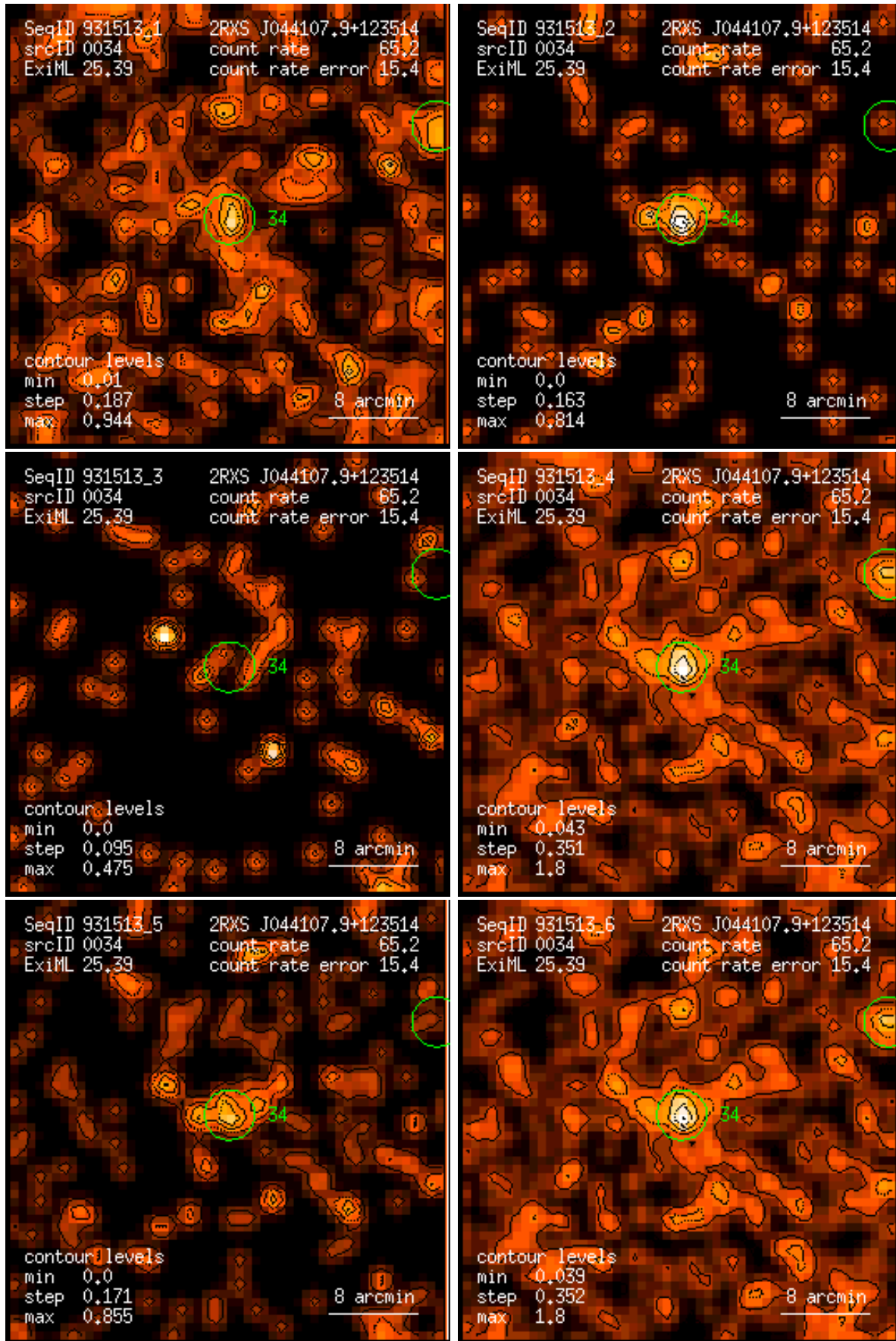
Figure 34: RASS 931513: detection 0034: band rate images, Gaussian filter: (1) PSPC channels 11 – 41, (2) 52 – 90, (3) 91 – 201, (4) 11 – 235, (5) 52 – 201, (6) 11 – 201. Broad band rates in counts/ks. Band rate contour levels in counts/ks/arcmin 2 .
