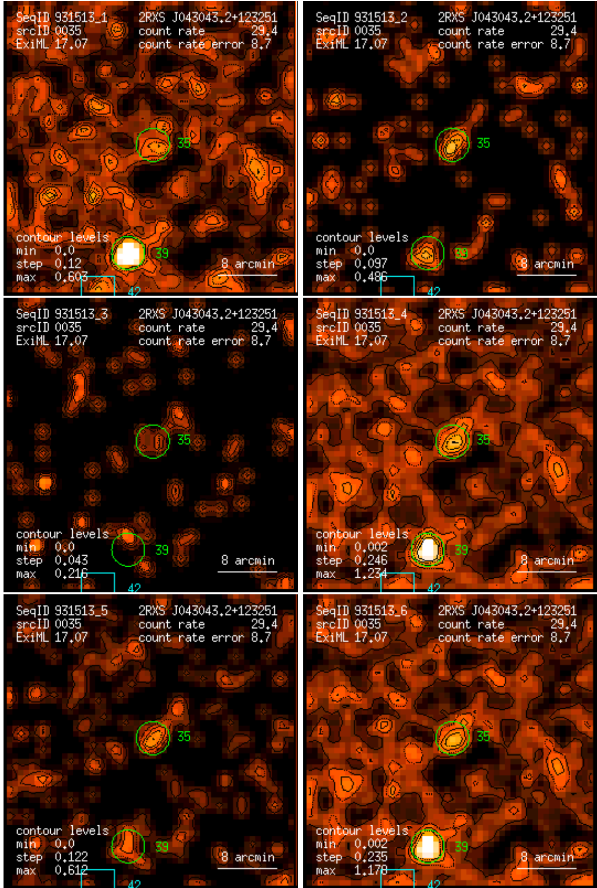
Figure 35: RASS 931513: detection 0035: band rate images, Gaussian filter: (1) PSPC channels 11 – 41, (2) 52 – 90, (3) 91 – 201, (4) 11 – 235, (5) 52 – 201, (6) 11 – 201. Broad band rates in counts/ks. Band rate contour levels in counts/ks/arcmin 2 .
