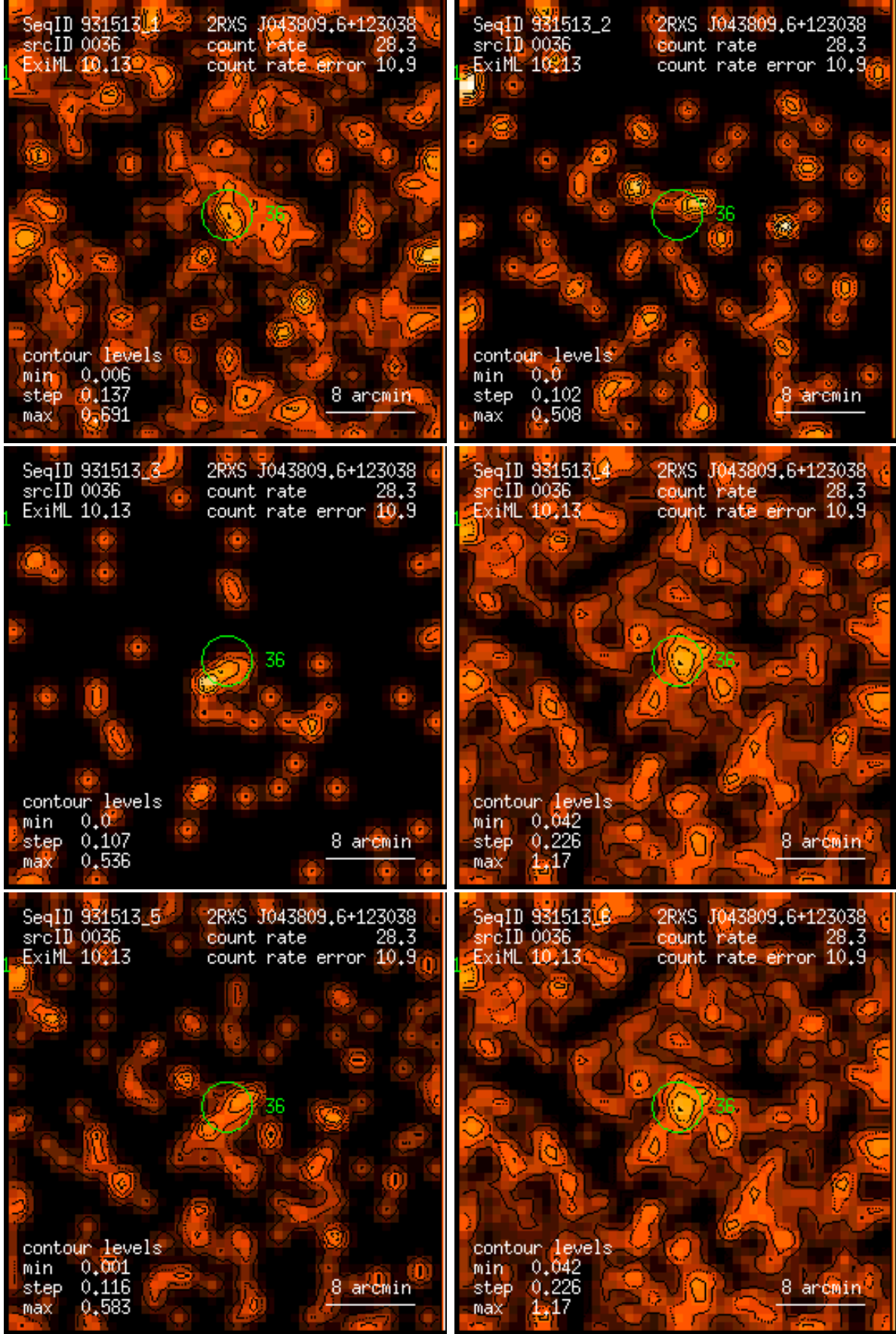
Figure 36: RASS 931513: detection 0036: band rate images, Gaussian filter: (1) PSPC channels 11 – 41, (2) 52 – 90, (3) 91 – 201, (4) 11 – 235, (5) 52 – 201, (6) 11 – 201. Broad band rates in counts/ks. Band rate contour levels in counts/ks/arcmin 2 .
