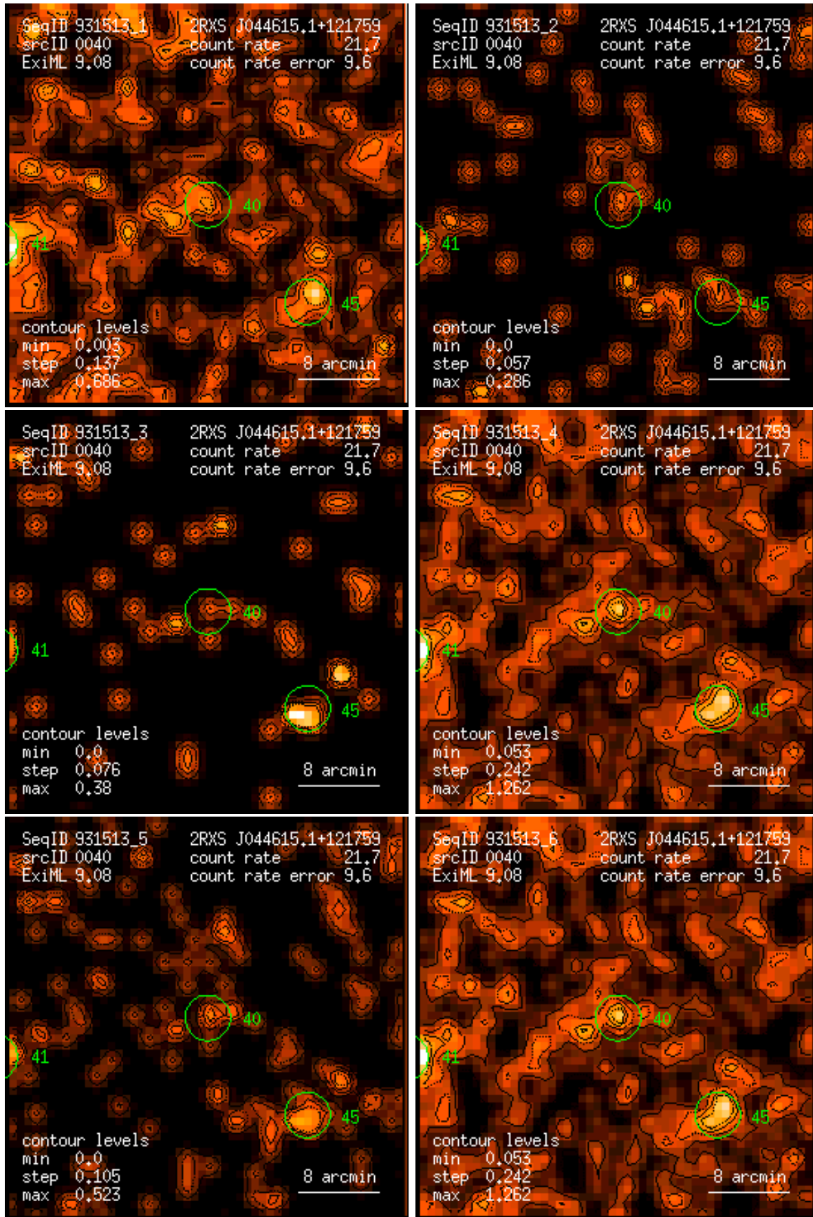
Figure 40: RASS 931513: detection 0040: band rate images, Gaussian filter: (1) PSPC channels 11 – 41, (2) 52 – 90, (3) 91 – 201, (4) 11 – 235, (5) 52 – 201, (6) 11 – 201. Broad band rates in counts/ks. Band rate contour levels in counts/ks/arcmin 2 .
