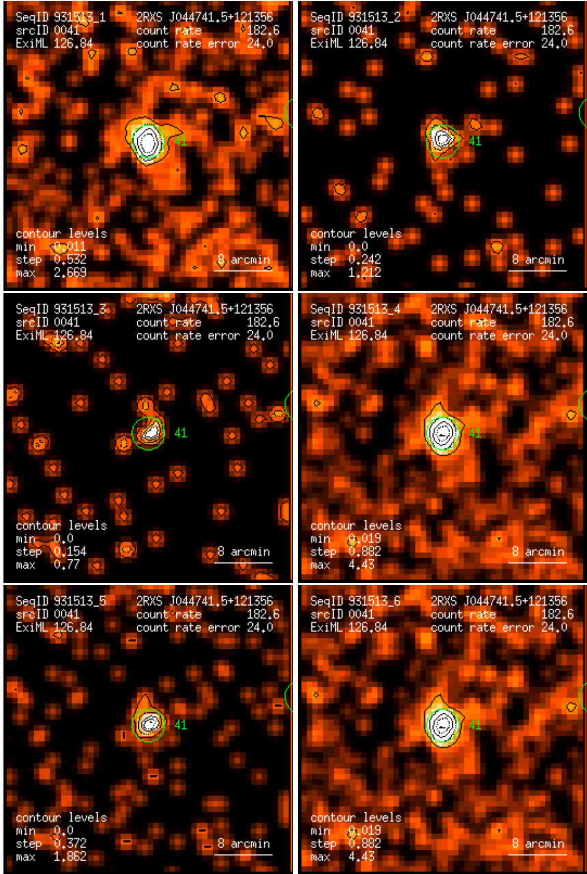
Figure 41: RASS 931513: detection 0041: band rate images, Gaussian filter: (1) PSPC channels 11 – 41, (2) 52 – 90, (3) 91 – 201, (4) 11 – 235, (5) 52 – 201, (6) 11 – 201. Broad band rates in counts/ks. Band rate contour levels in counts/ks/arcmin 2 .
