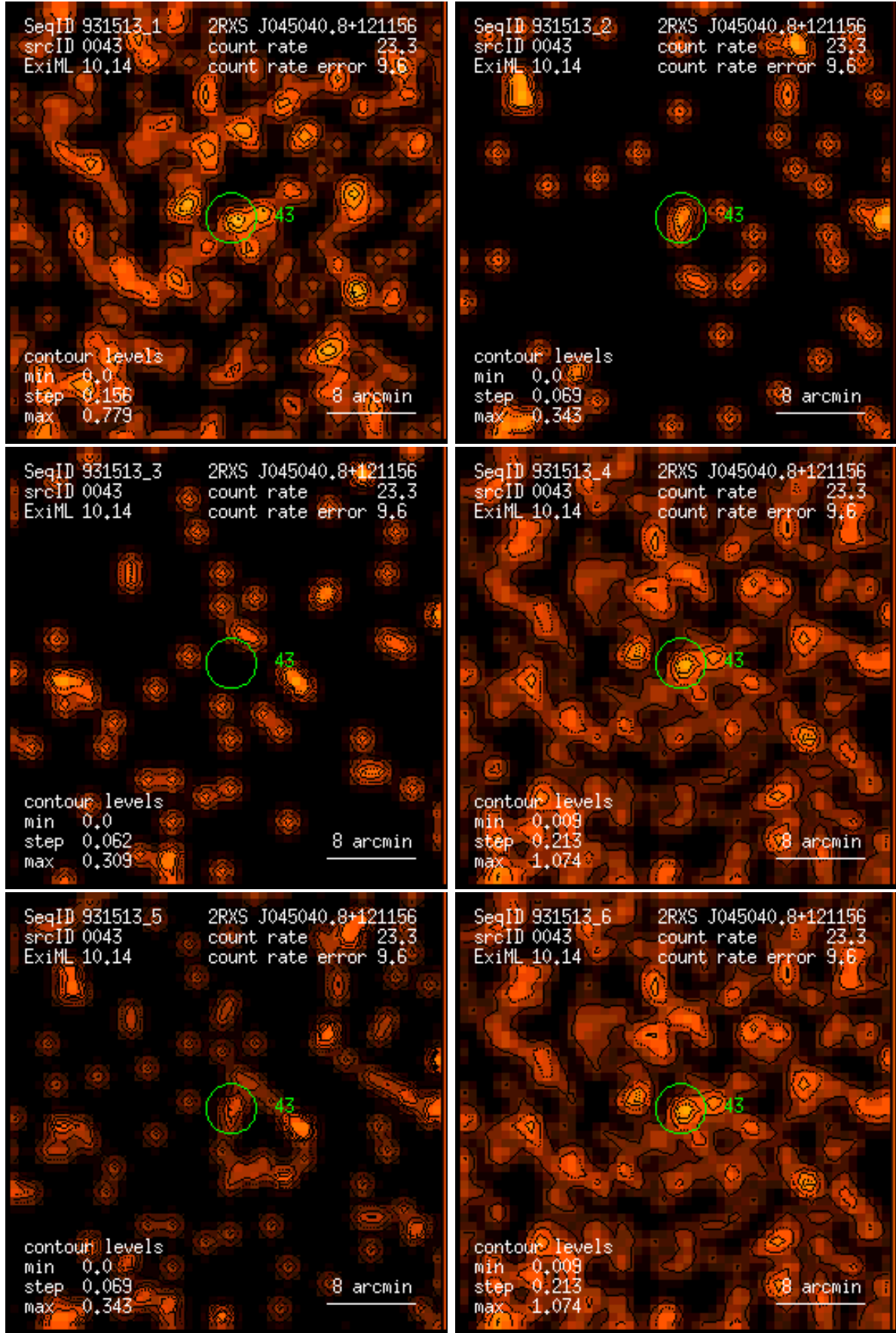
Figure 43: RASS 931513: detection 0043: band rate images, Gaussian filter: (1) PSPC channels 11 – 41, (2) 52 – 90, (3) 91 – 201, (4) 11 – 235, (5) 52 – 201, (6) 11 – 201. Broad band rates in counts/ks. Band rate contour levels in counts/ks/arcmin 2 .
