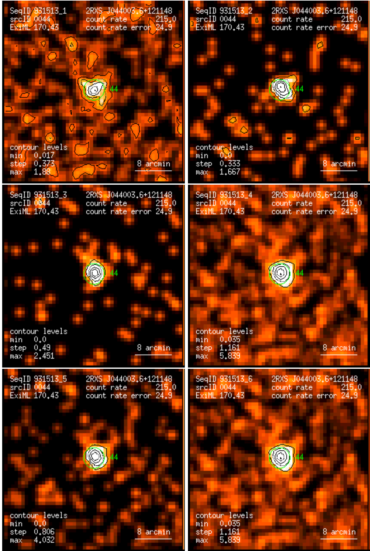
Figure 44: RASS 931513: detection 0044: band rate images, Gaussian filter: (1) PSPC channels 11 – 41, (2) 52 – 90, (3) 91 – 201, (4) 11 – 235, (5) 52 – 201, (6) 11 – 201. Broad band rates in counts/ks. Band rate contour levels in counts/ks/arcmin 2 .
