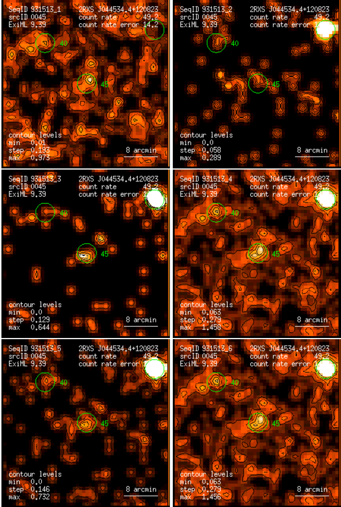
Figure 45: RASS 931513: detection 0045: band rate images, Gaussian filter: (1) PSPC channels 11 – 41, (2) 52 – 90, (3) 91 – 201, (4) 11 – 235, (5) 52 – 201, (6) 11 – 201. Broad band rates in counts/ks. Band rate contour levels in counts/ks/arcmin 2 .
