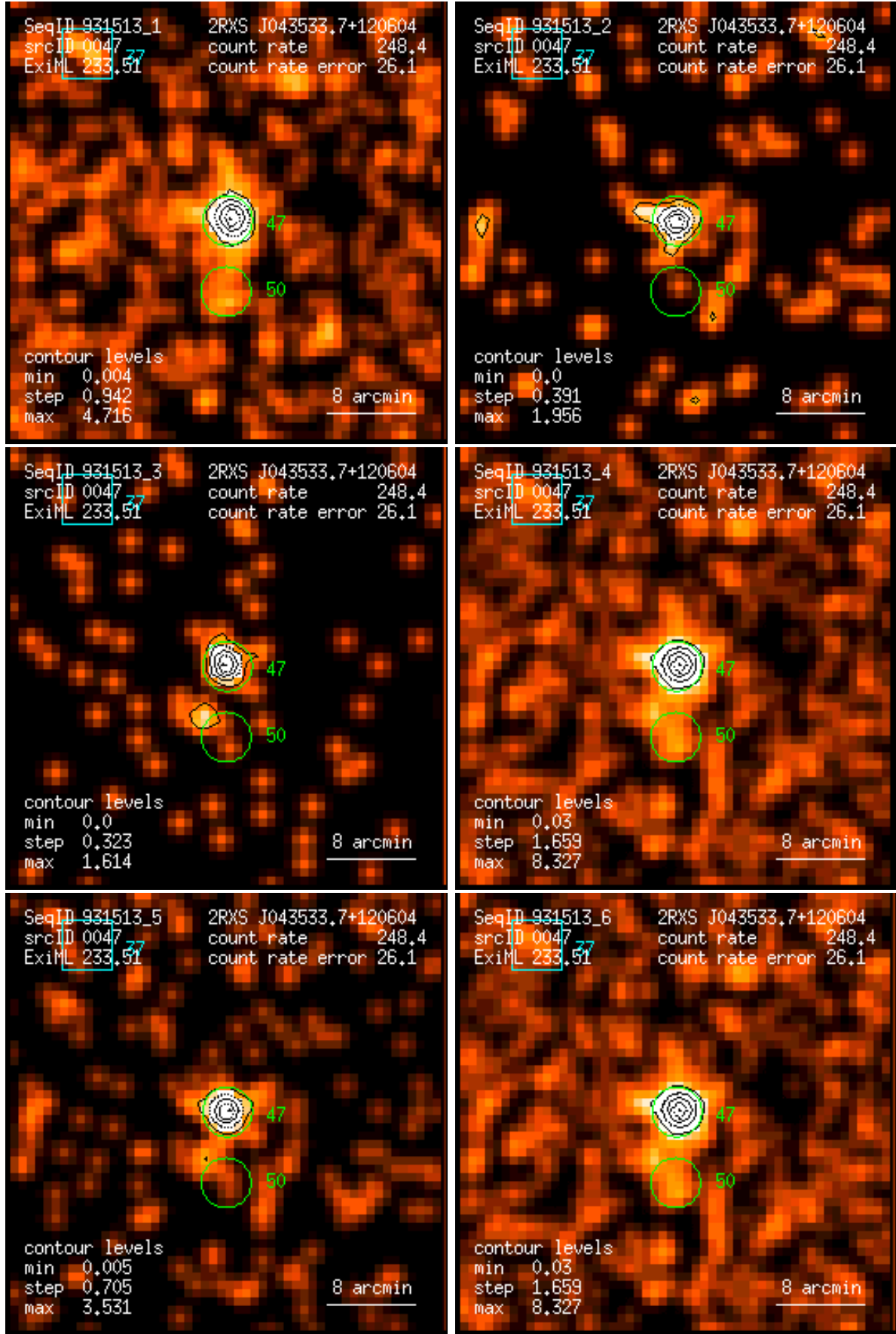
Figure 47: RASS 931513: detection 0047: band rate images, Gaussian filter: (1) PSPC channels 11 – 41, (2) 52 – 90, (3) 91 – 201, (4) 11 – 235, (5) 52 – 201, (6) 11 – 201. Broad band rates in counts/ks. Band rate contour levels in counts/ks/arcmin 2 .
