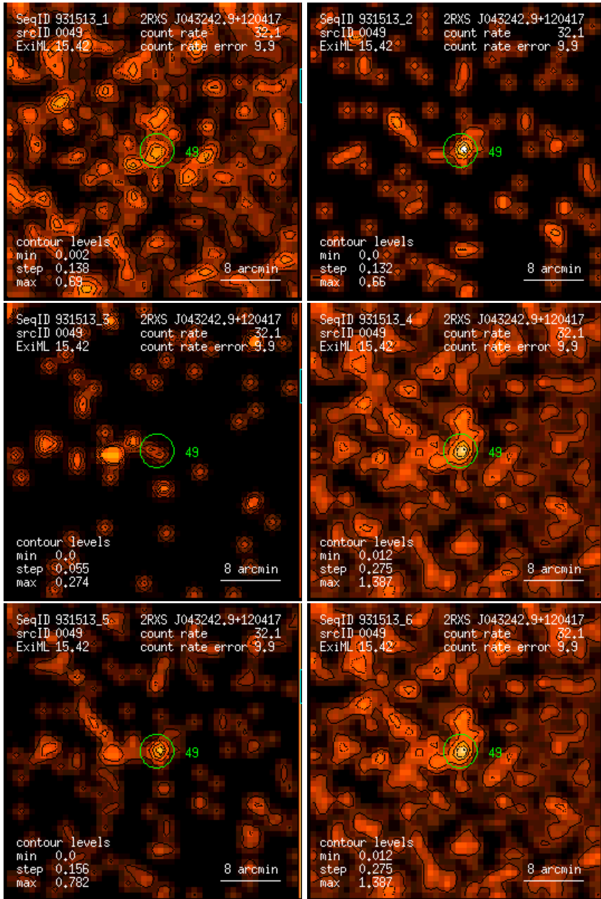
Figure 49: RASS 931513: detection 0049: band rate images, Gaussian filter: (1) PSPC channels 11 – 41, (2) 52 – 90, (3) 91 – 201, (4) 11 – 235, (5) 52 – 201, (6) 11 – 201. Broad band rates in counts/ks. Band rate contour levels in counts/ks/arcmin 2 .
